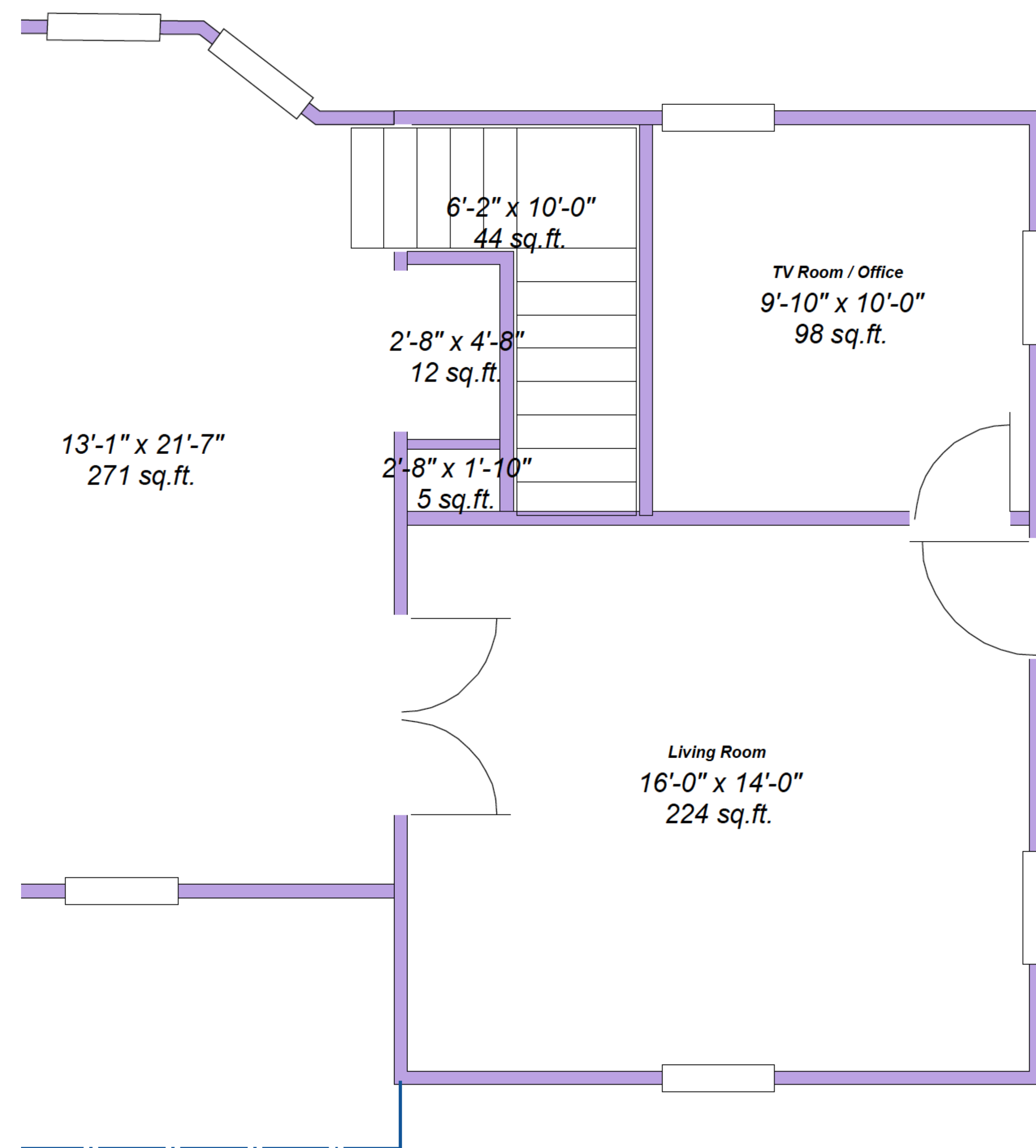
Proposed First Floor Renovation Layout
