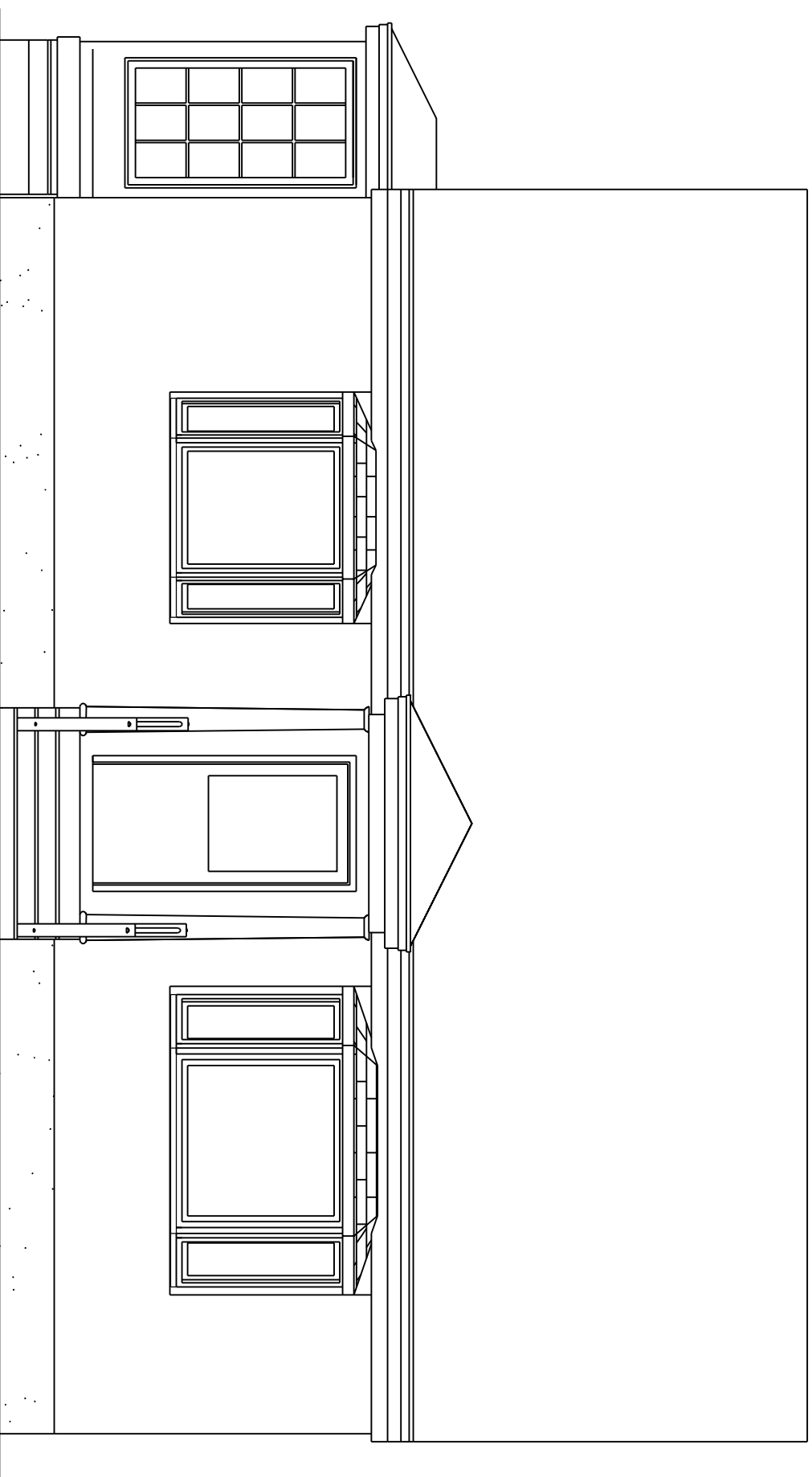
4 WEST ELEVATION 1/4" = 1'-0"
