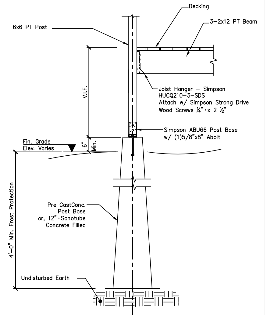
SECTION 3 AT PRECAST CONCRETE PIER Scale: 1/2" = 1'-0"
