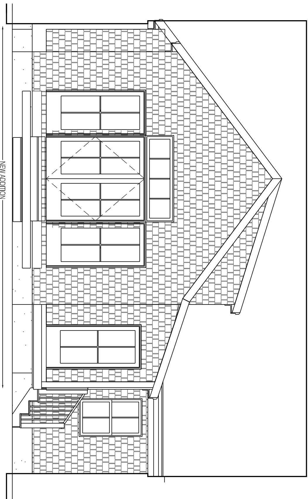
2 WEST ELEVATION 1/4" = 1'-0"
