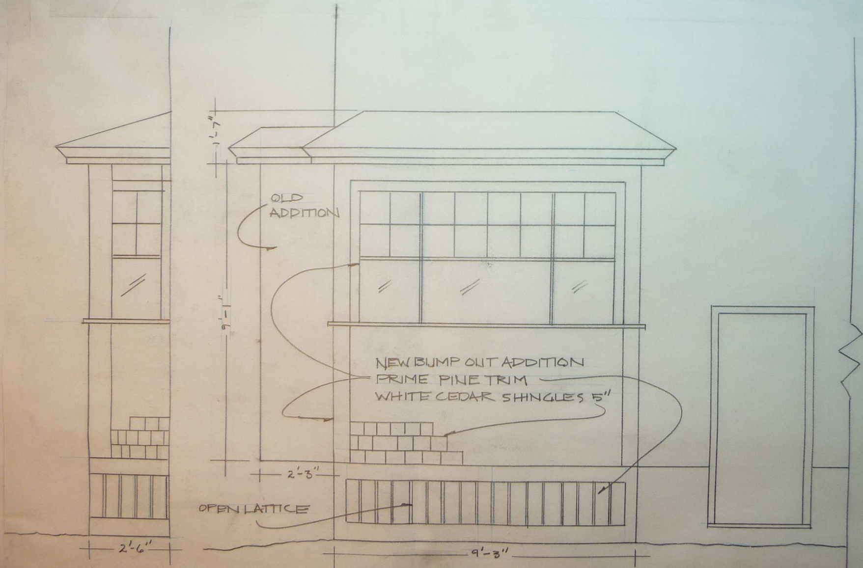
North Kitchen Elev. SCALE: 1/2" = 1'-0"
