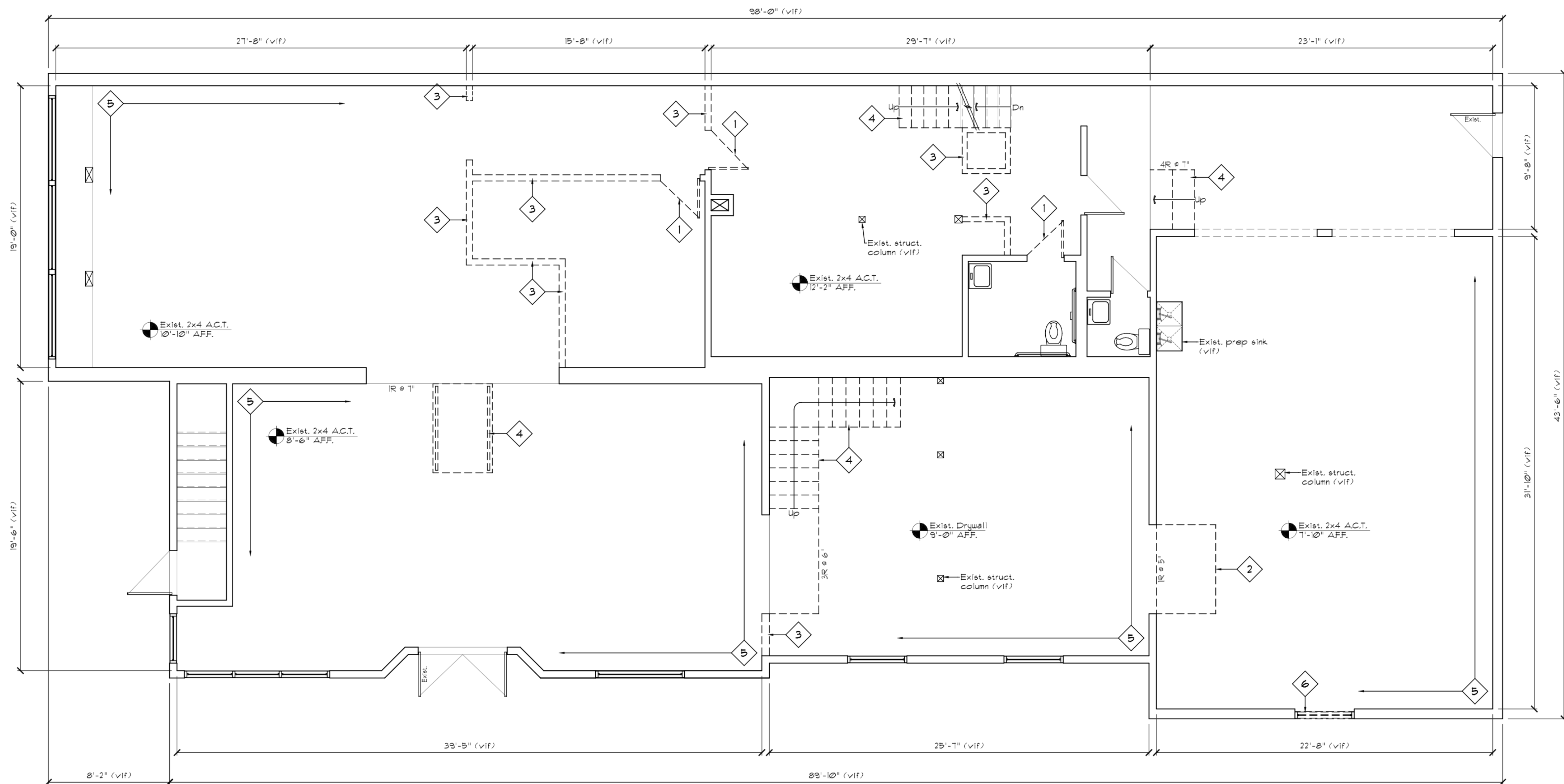
1 Existing/ Demolition Plan D-1 SCALE: 1/4" = 1'-0"
