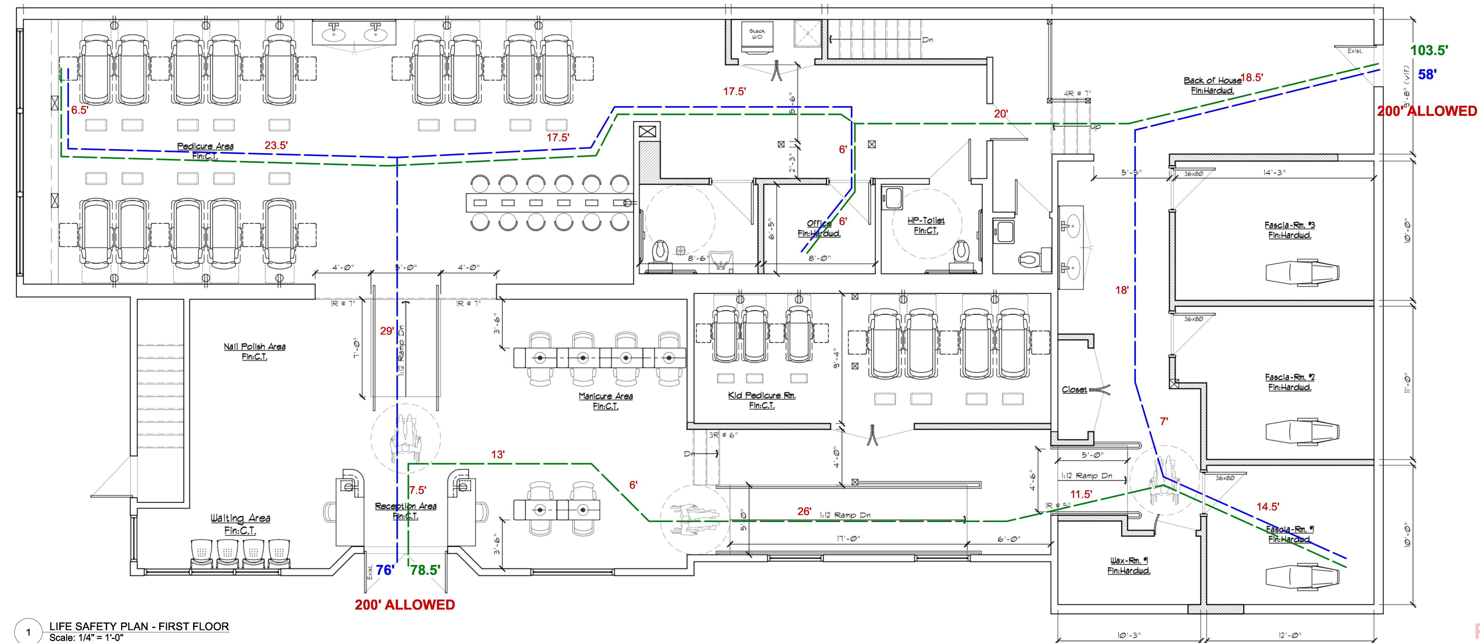
2 LIFE SAFETY PLAN - SECOND FLOOR Scale: 1/4" = 1'-0"
