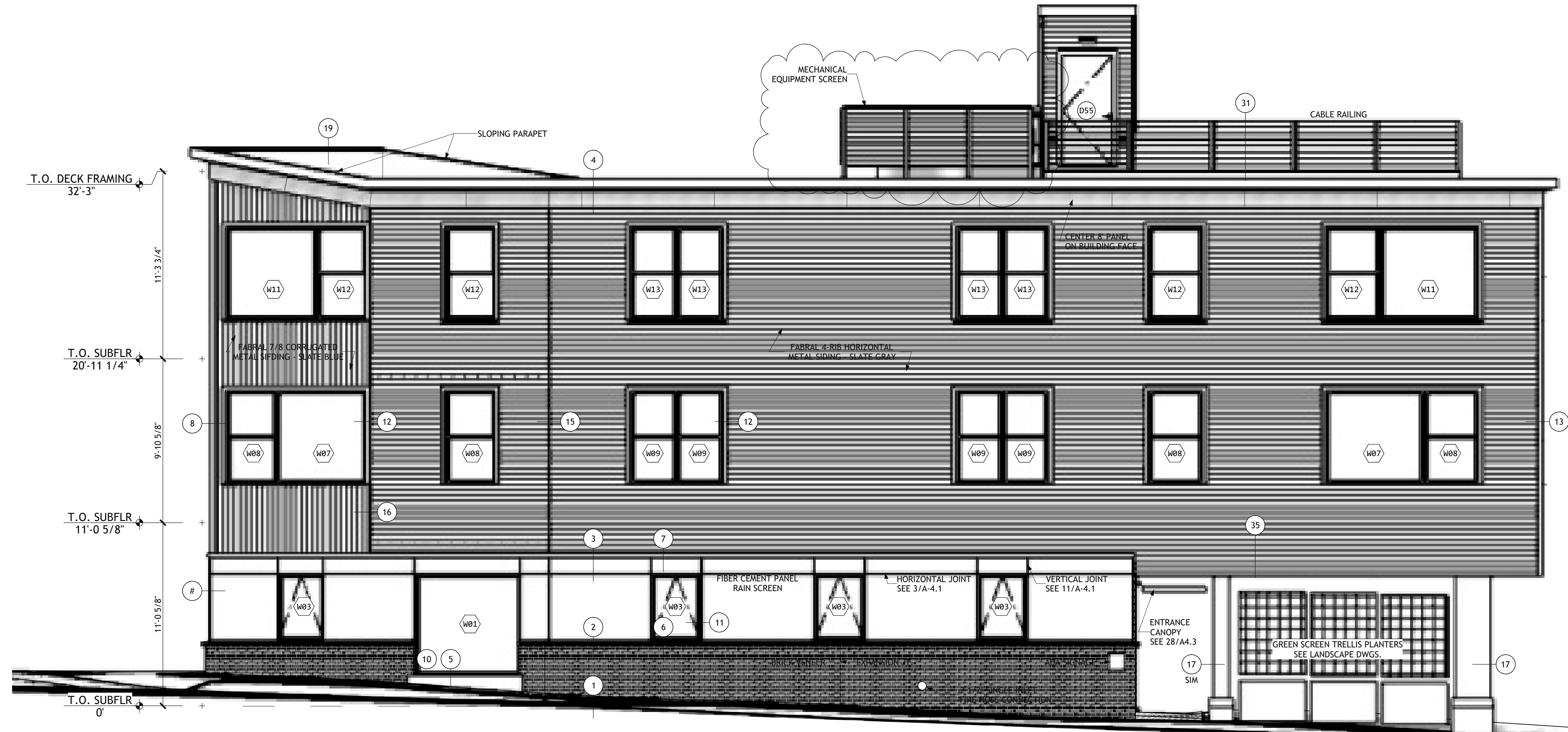
2 : South Elevation : 1/4 in = 1 ft
