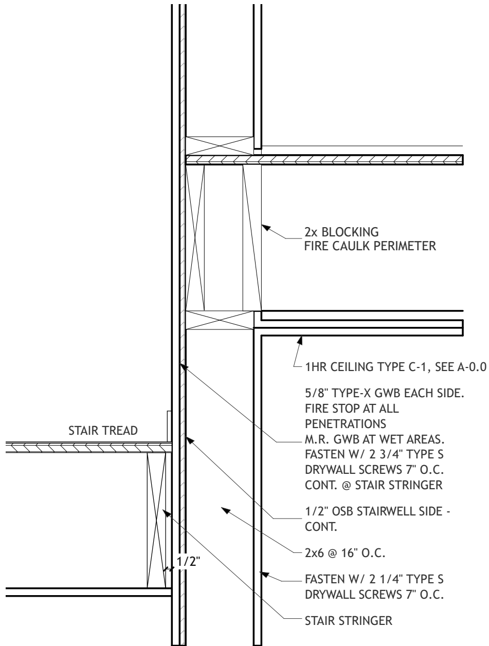
1 HOUR WALL IBC 14-1.14 W/ STRUCTURAL WOOD PANEL @ STAIR STRINGER
