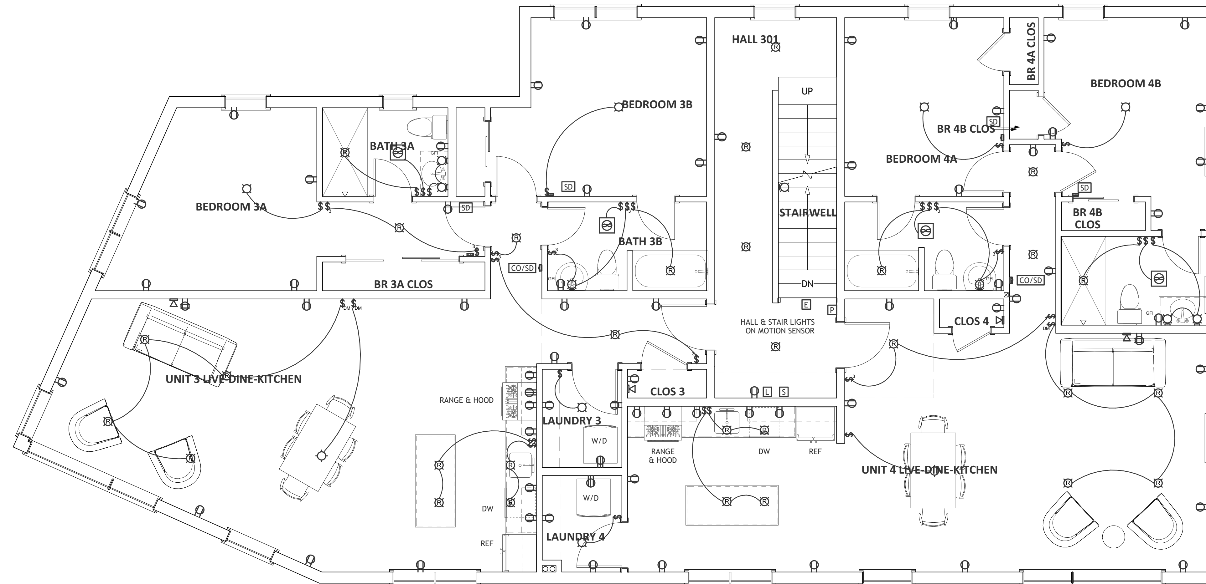
1 : Third Floor Electrical Plan : 1/4 in = 1 ft
