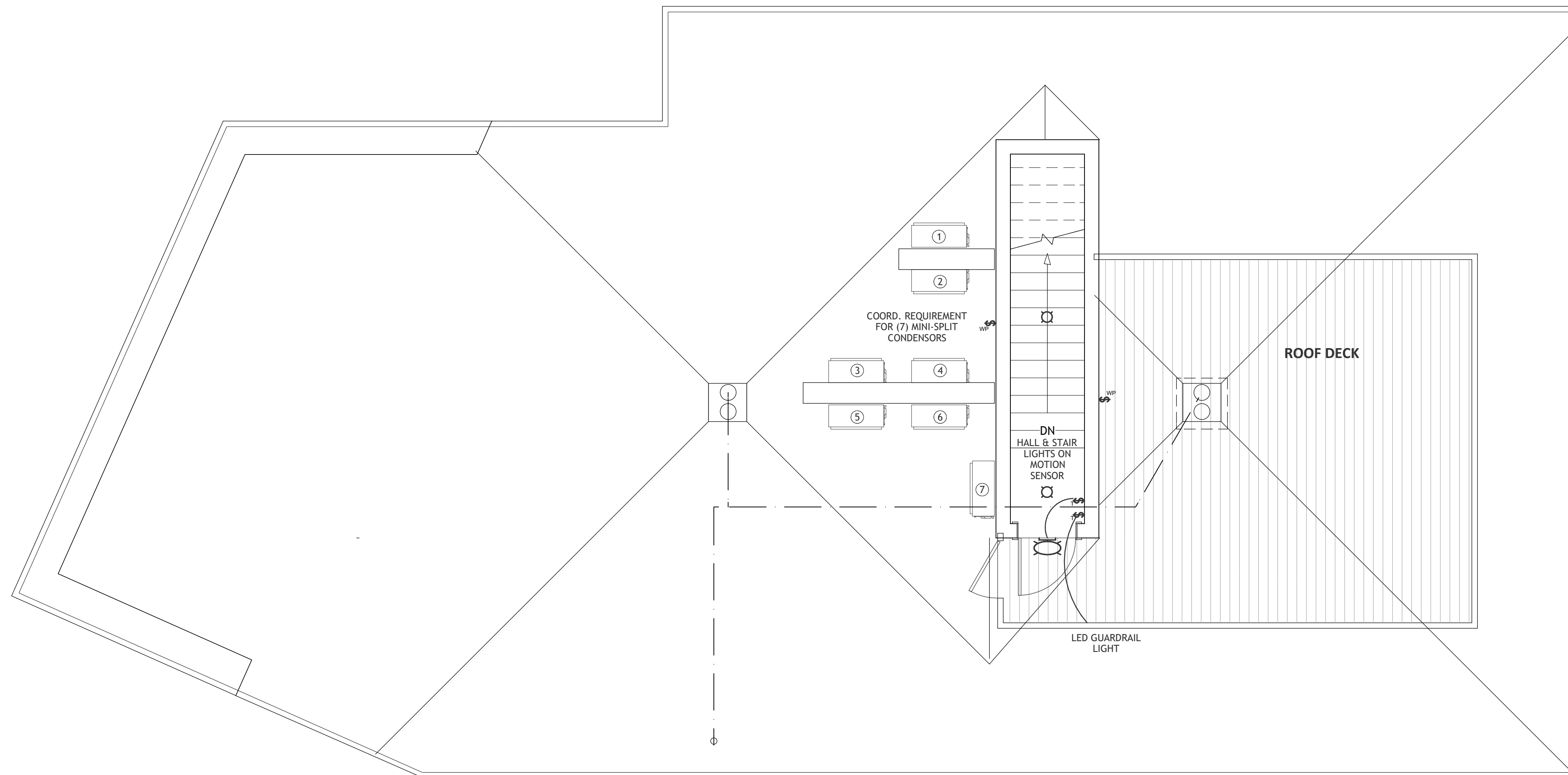
1 :Roof Electrical Plan : 1/4 in = 1 ft
