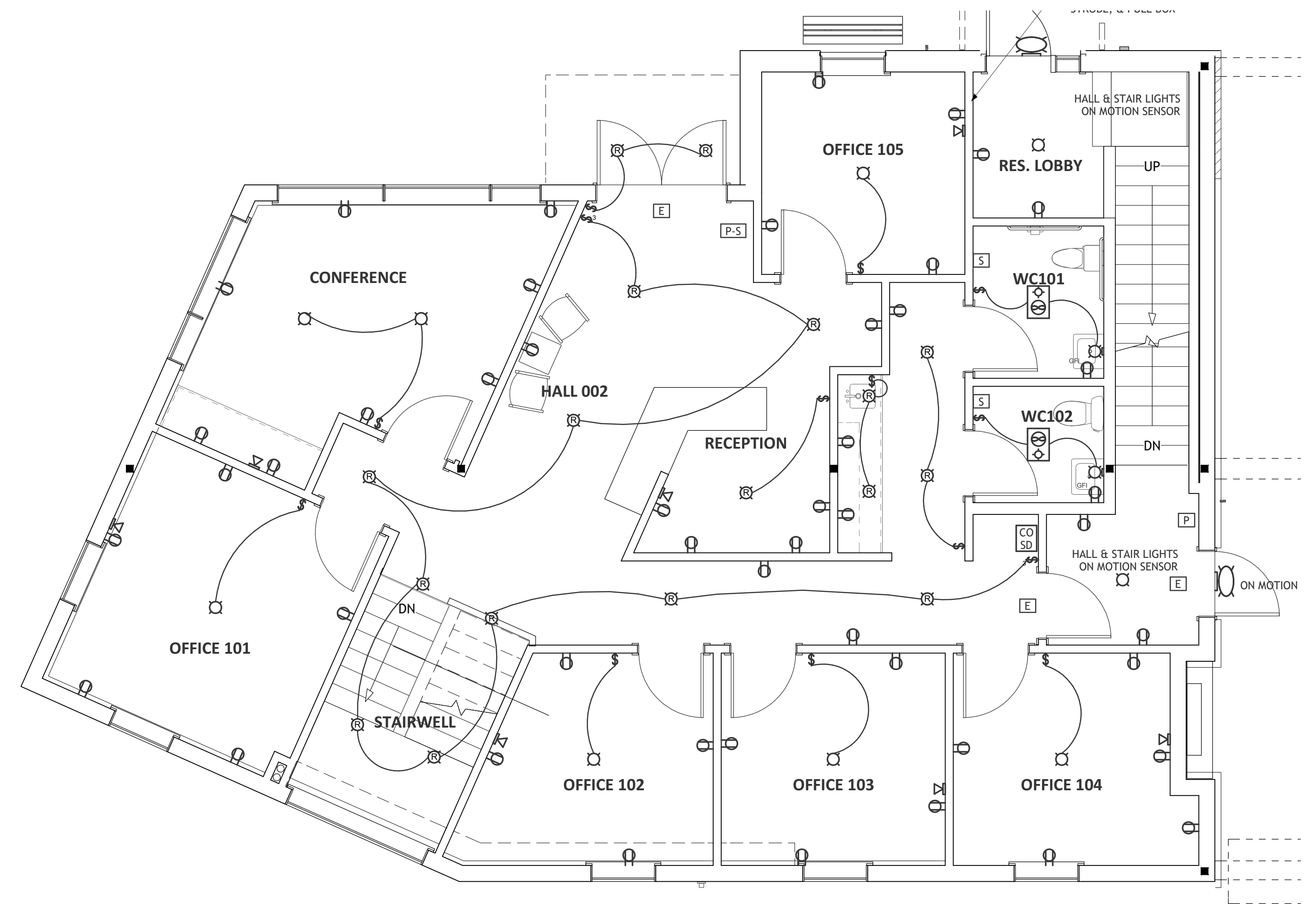
1 : First Floor Electrical Plan : 1/4 in = 1 ft
