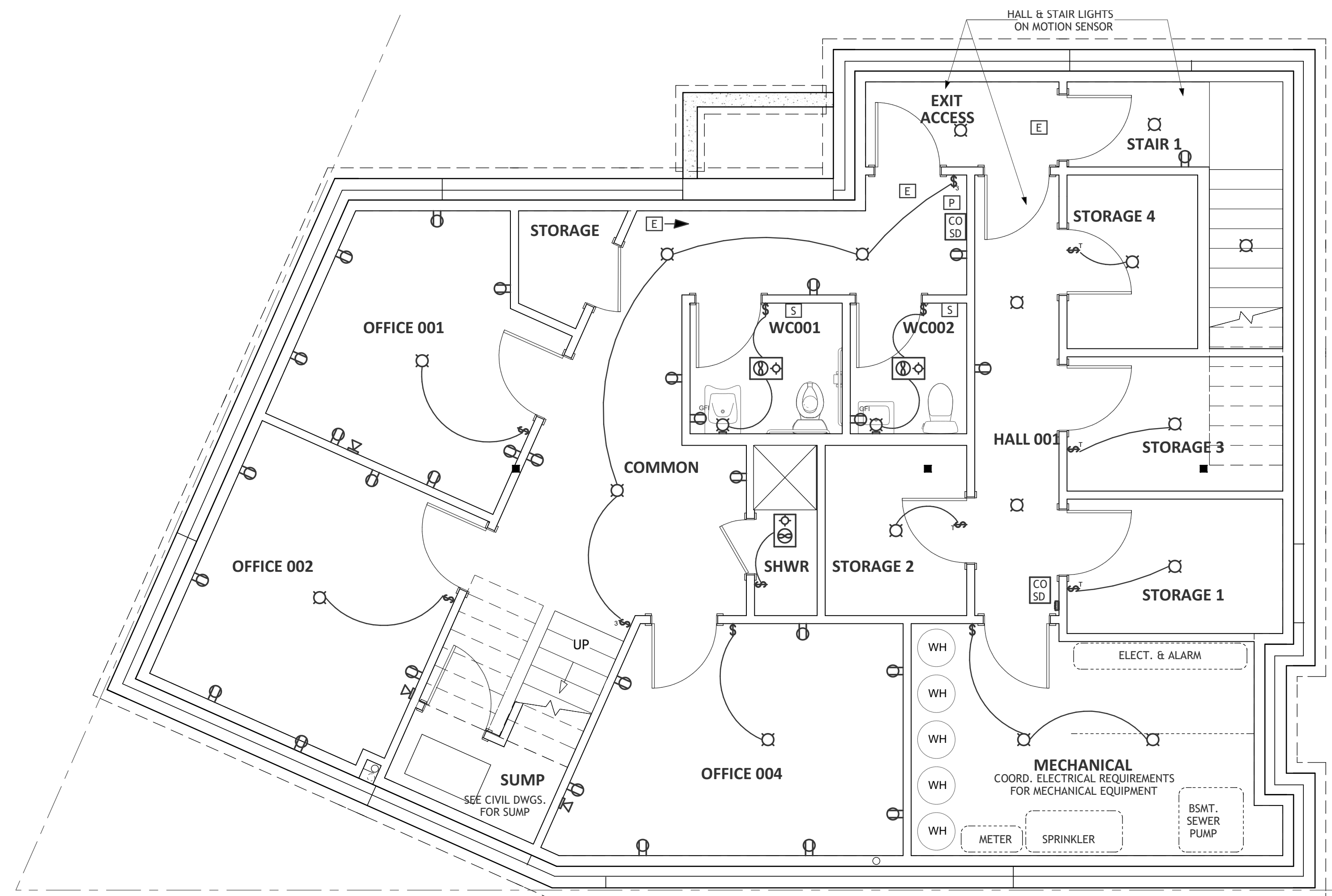
2 : Basement Electrical Plan : 1/4 in = 1 ft
