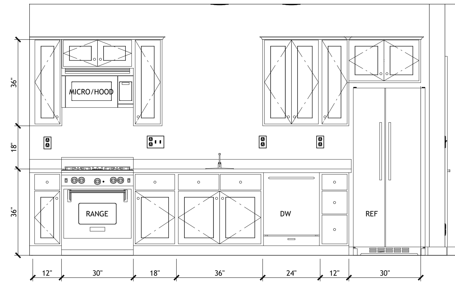
2 : Kitchen Elevation : 1/2 in = 1 ft
