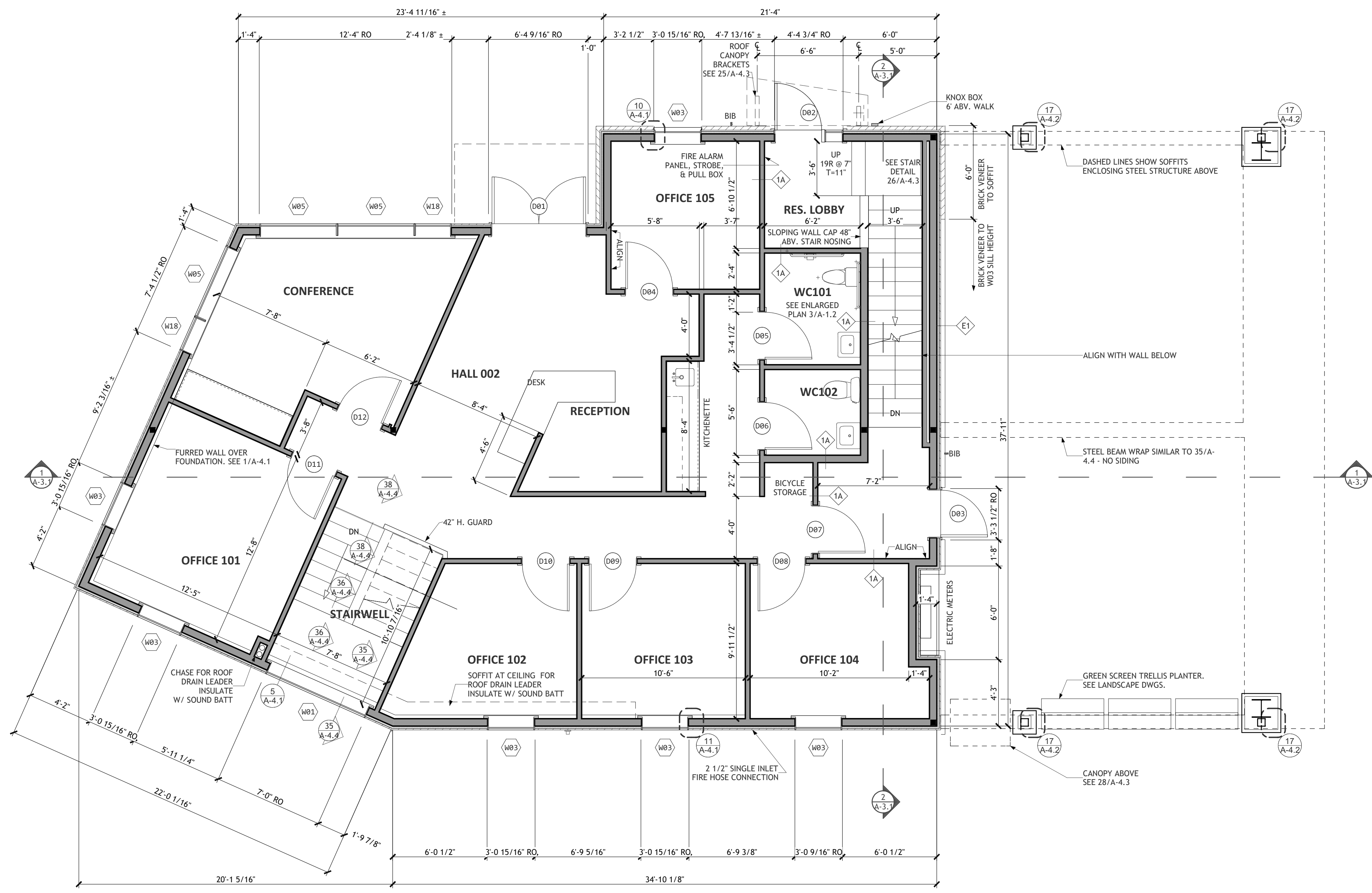
1 : First Floor Plan : 1/4 in = 1 ft
