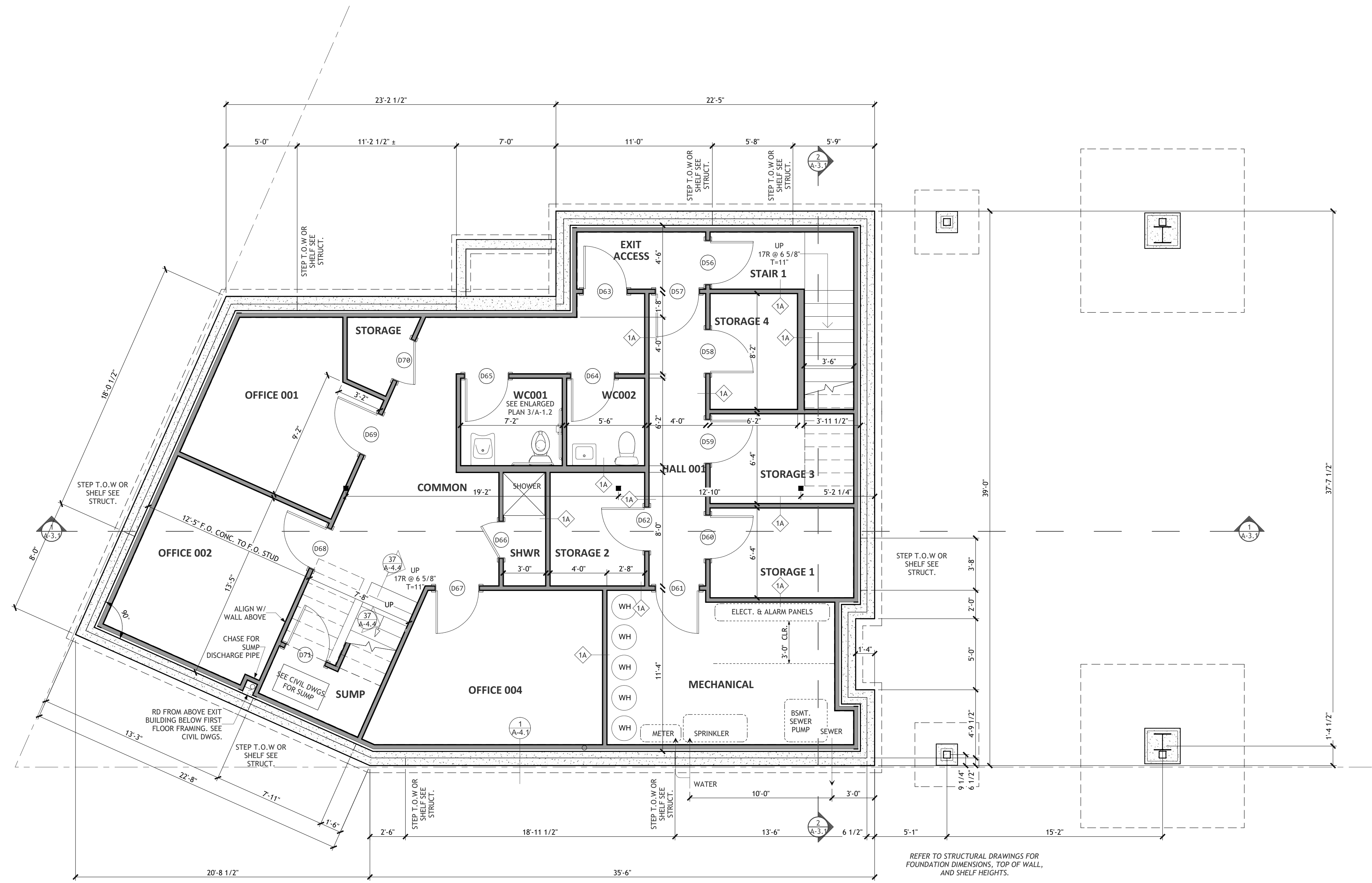
1 : Basement Plan : 1/4 in = 1 ft
