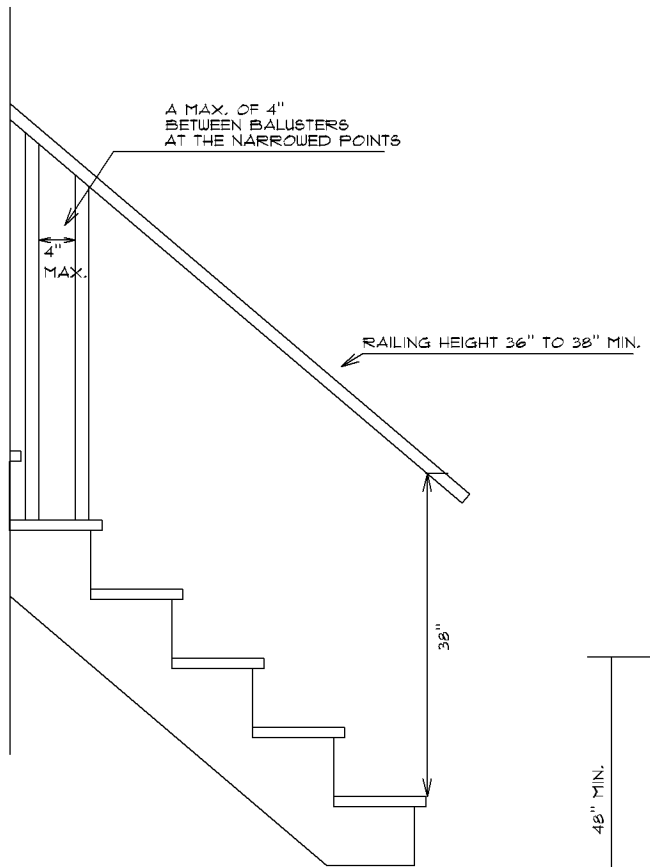
EXISTING STAIRS WITH NEW RAILINGS
