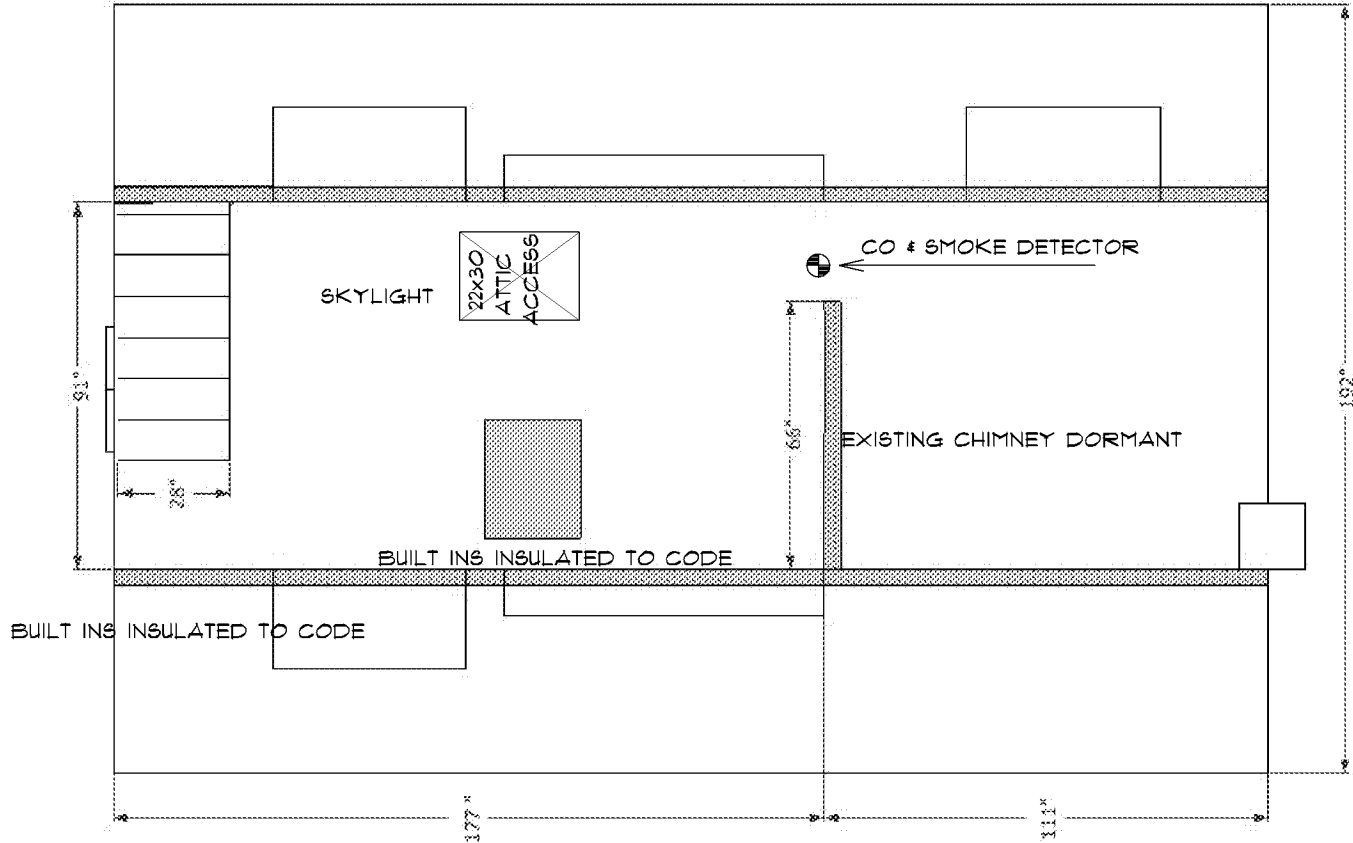
ATTIC FLOOR PLAN 1/4" = 1'
