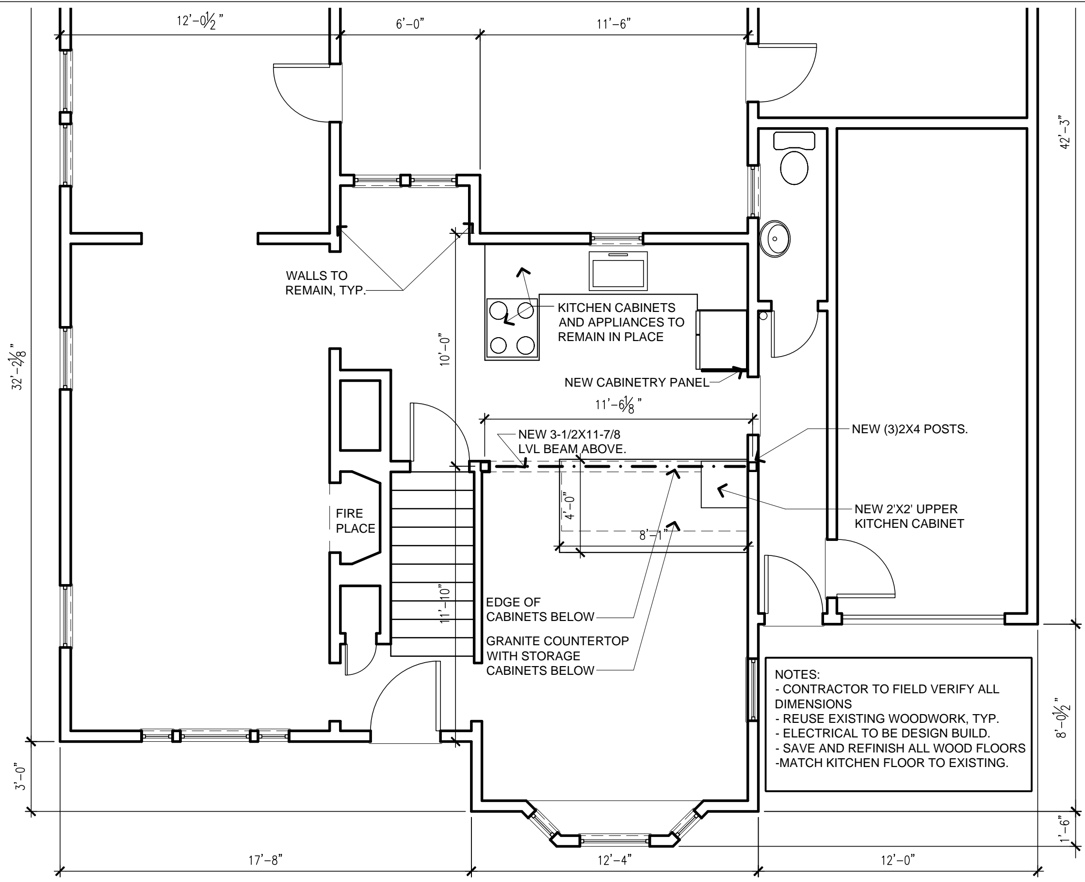
1 DEMO AND PROPOSED FIRST FLOOR PLAN SCALE - 1/4" = 1'-0"
