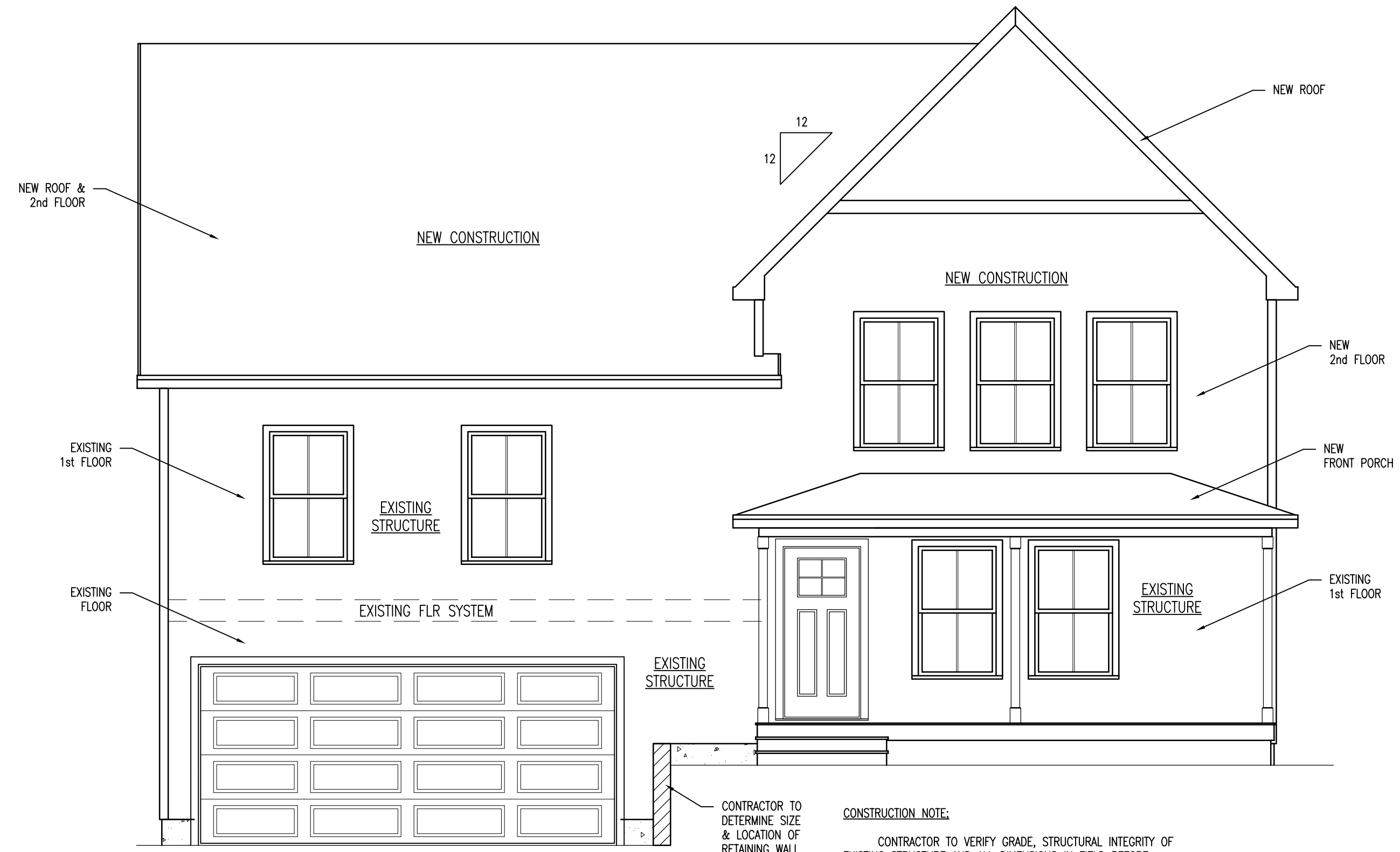
FRONT ELEVATION 1/4" = 1'-0"
