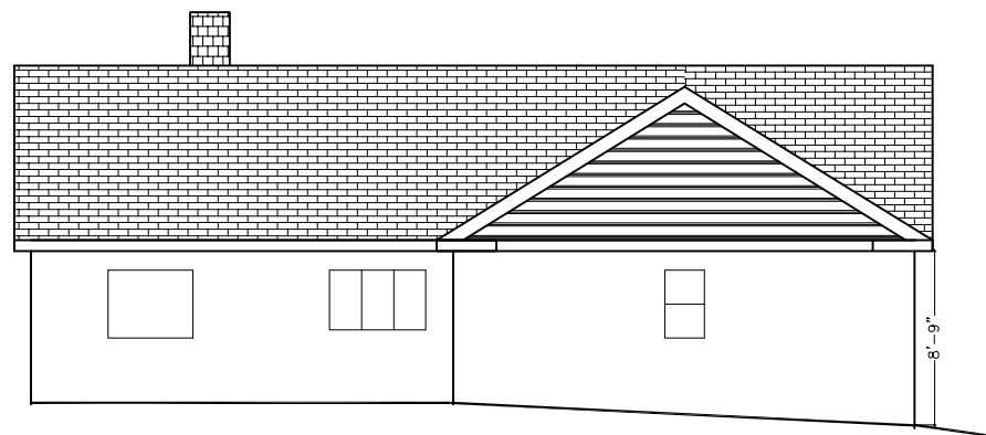
EXISTING LEFT ELEVATION SCALE: 3/32" = 1'-0"
