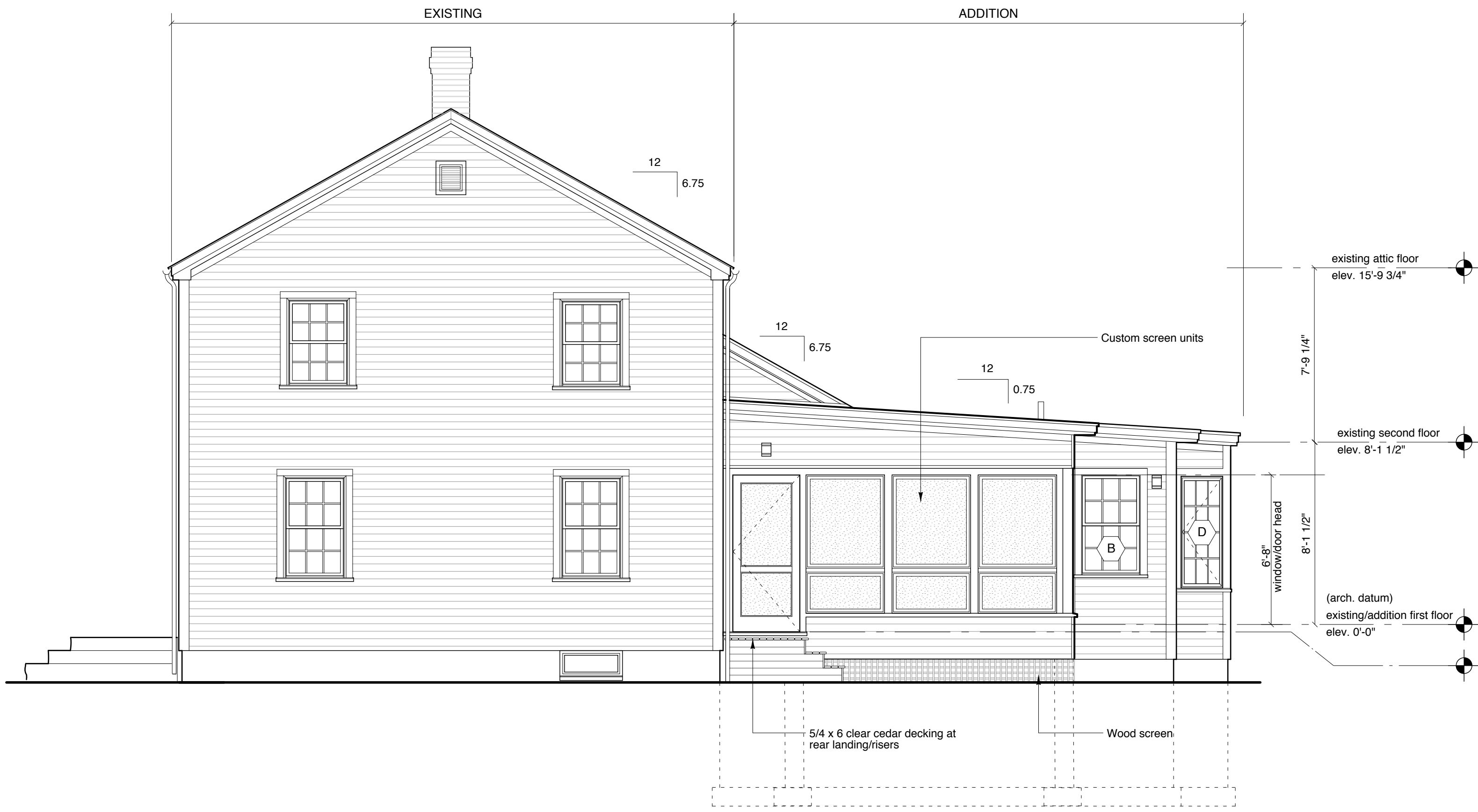
4 East Elevation SCALE: 1/4" = 1'-0"
