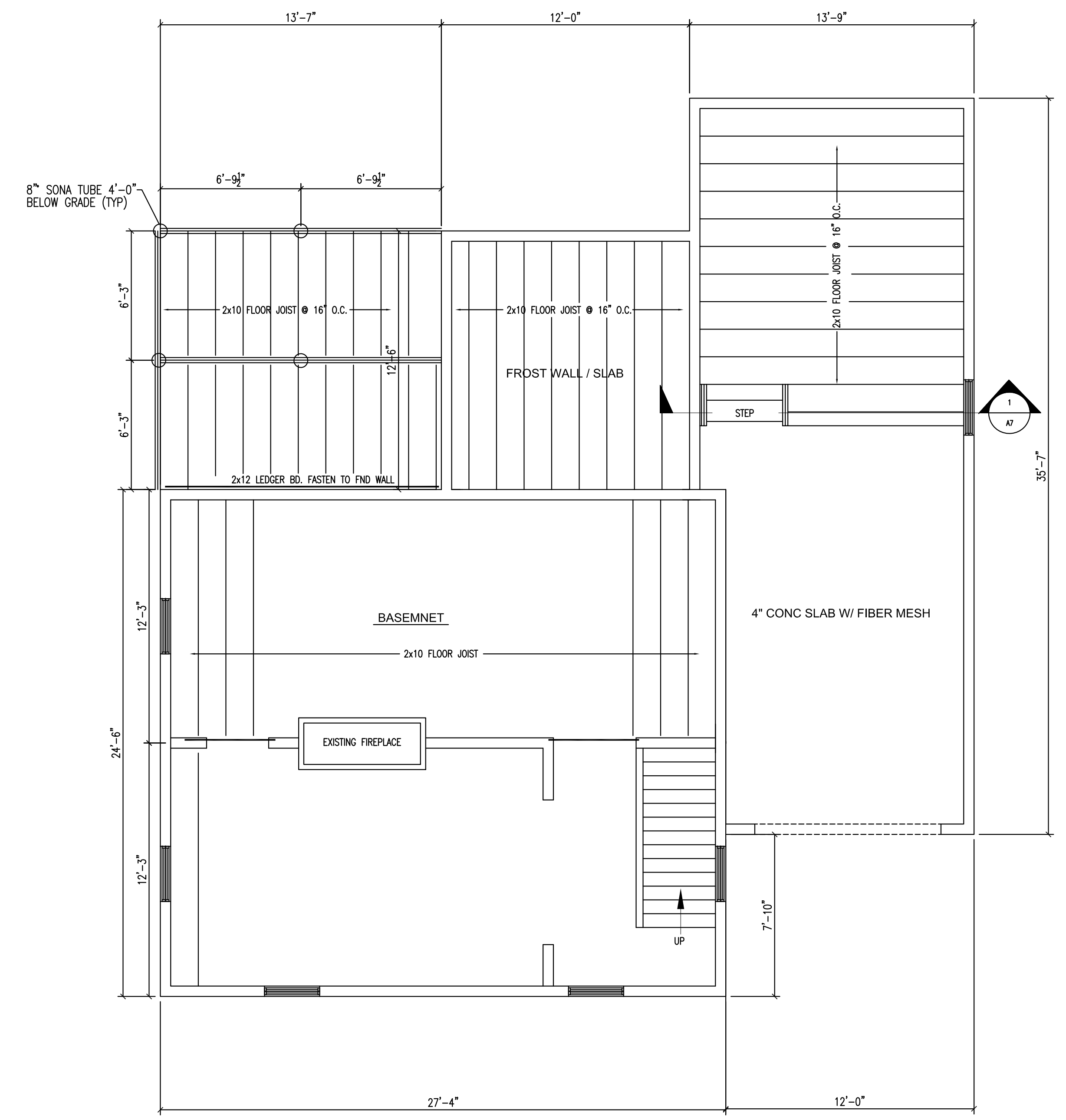
EXISTING & PROPOSED FOUNDATION PLAN 1/4"=1'-0"
