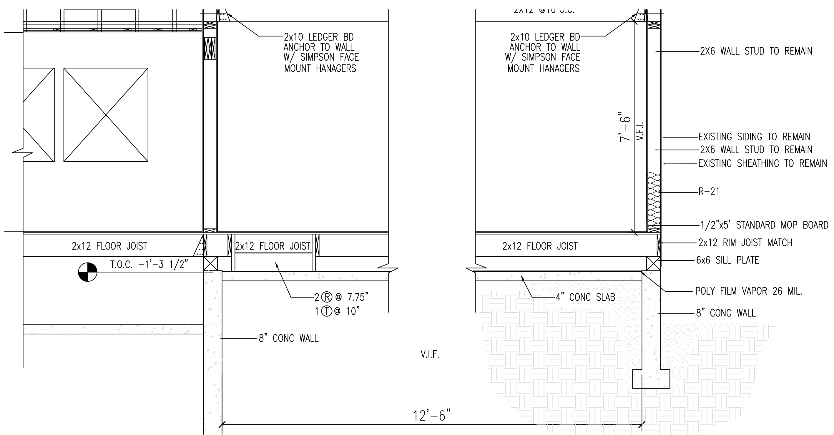
1 CROSS SECTION @ CAR PORT A4 1/2"=1'-0"
