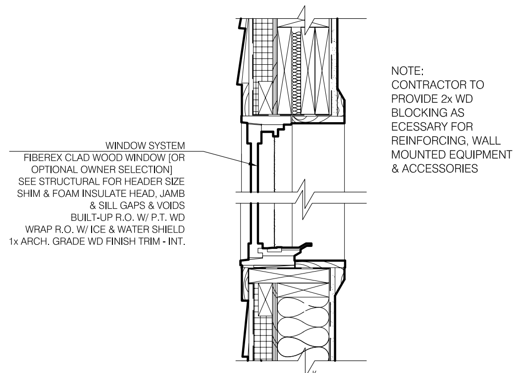
20 WINDOW SECTION 1 1/2" = 1'-0"
