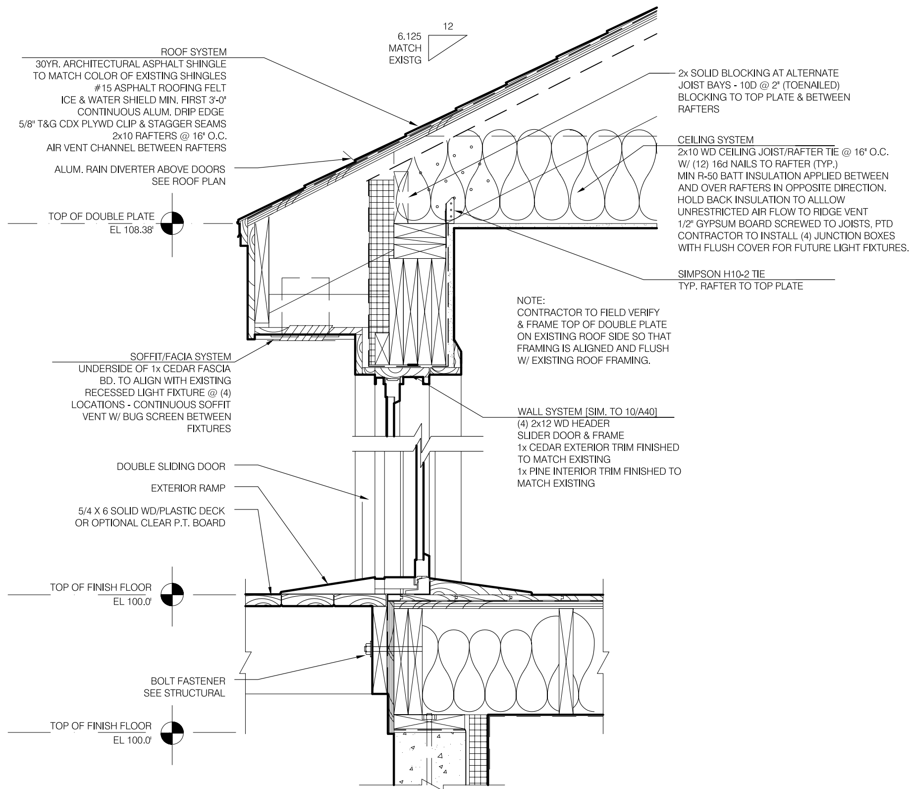
30 ROOF EAVE & DOOR FRAME DETAIL 1 1/2" = 1'-0"
