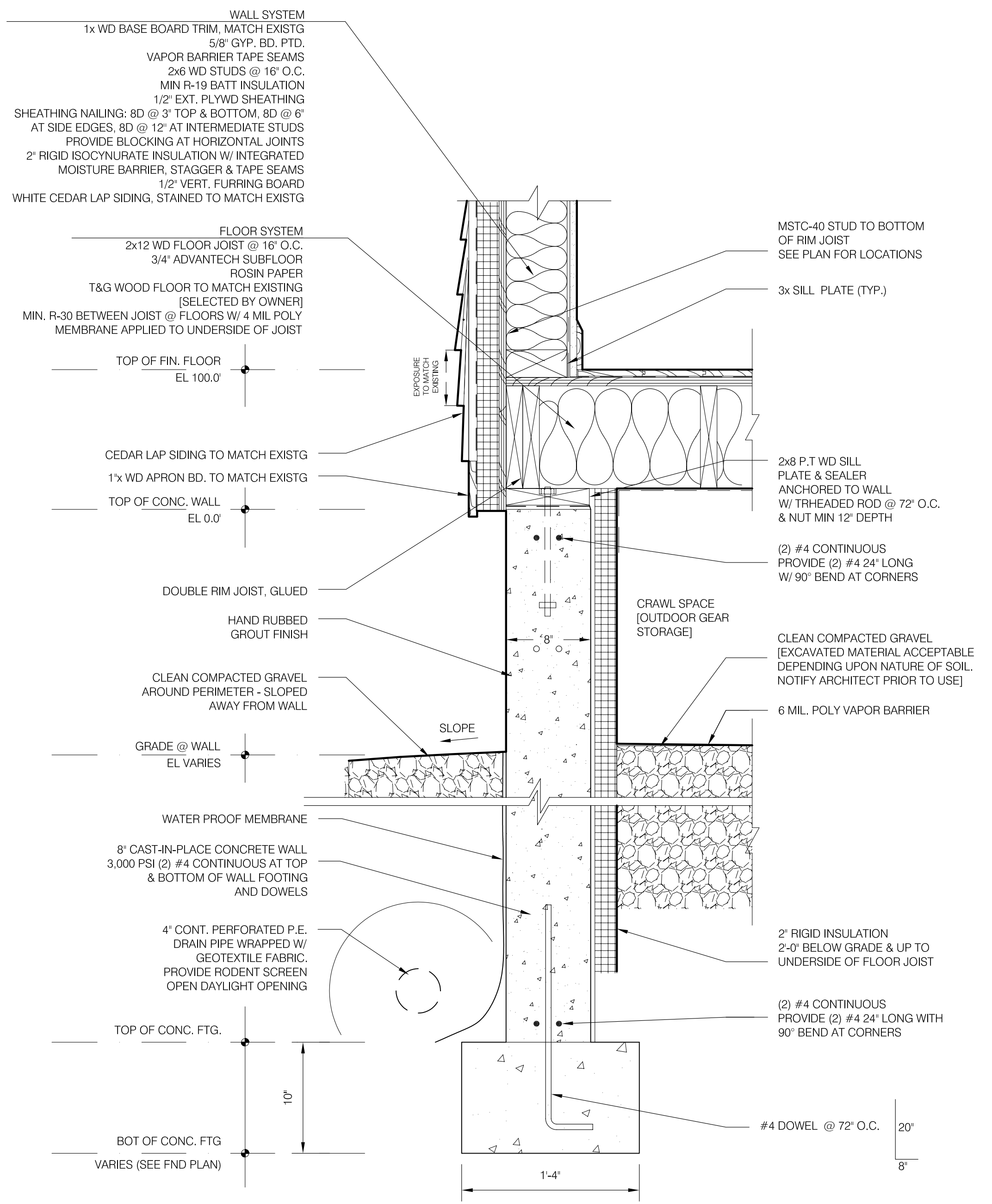
10 FOUNDATION WALL SECTION 1 1/2" = 1'-0"
