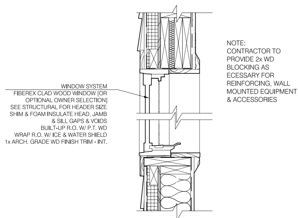
20 WINDOW SECTION 1 1/2" = 1'-0"
