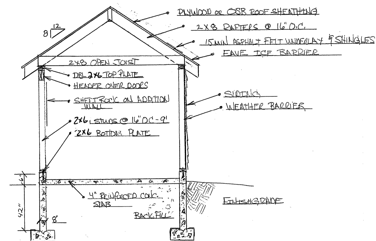
GARAGE SECTION
