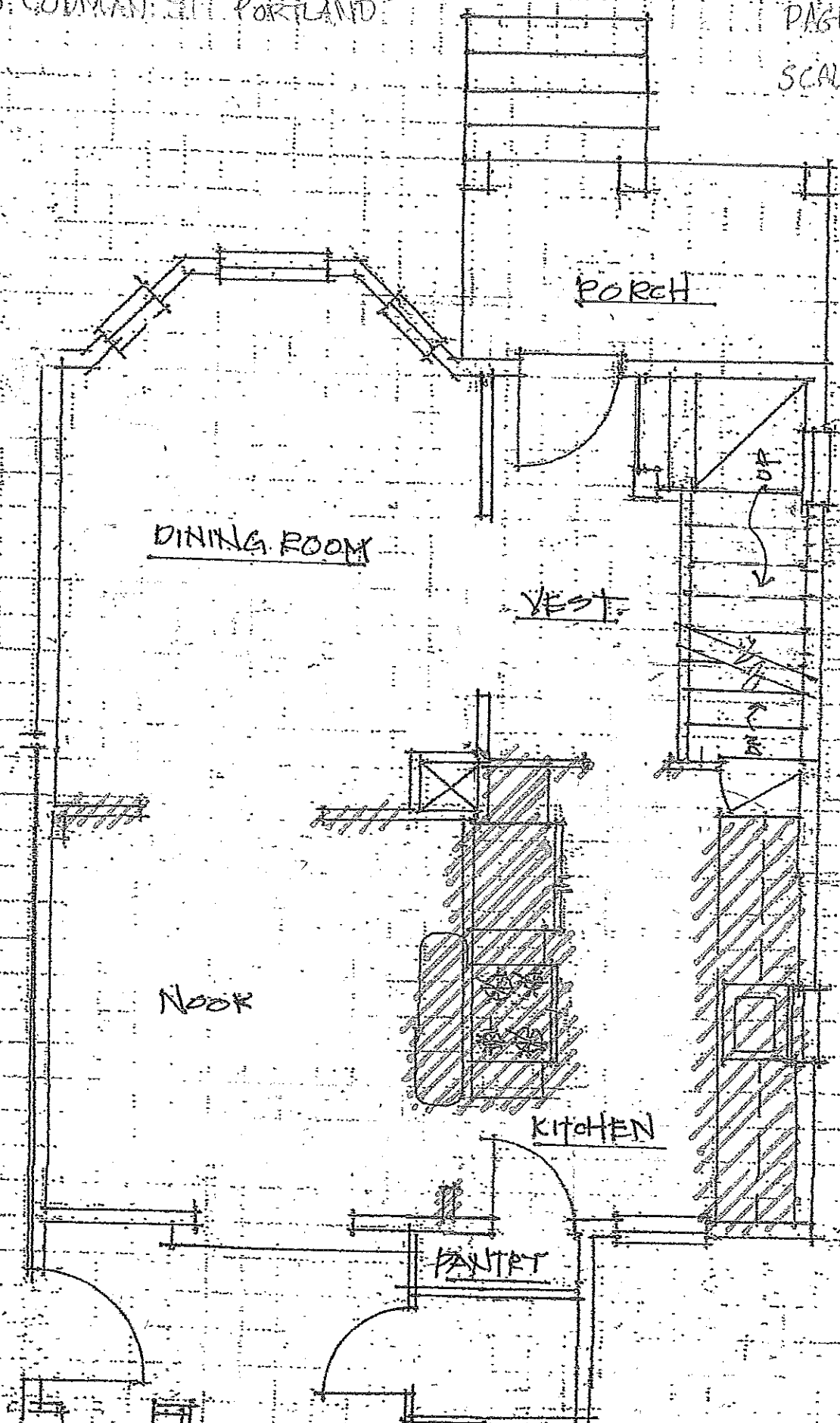
FIRST FLOOR DEMOLITION PLAN
