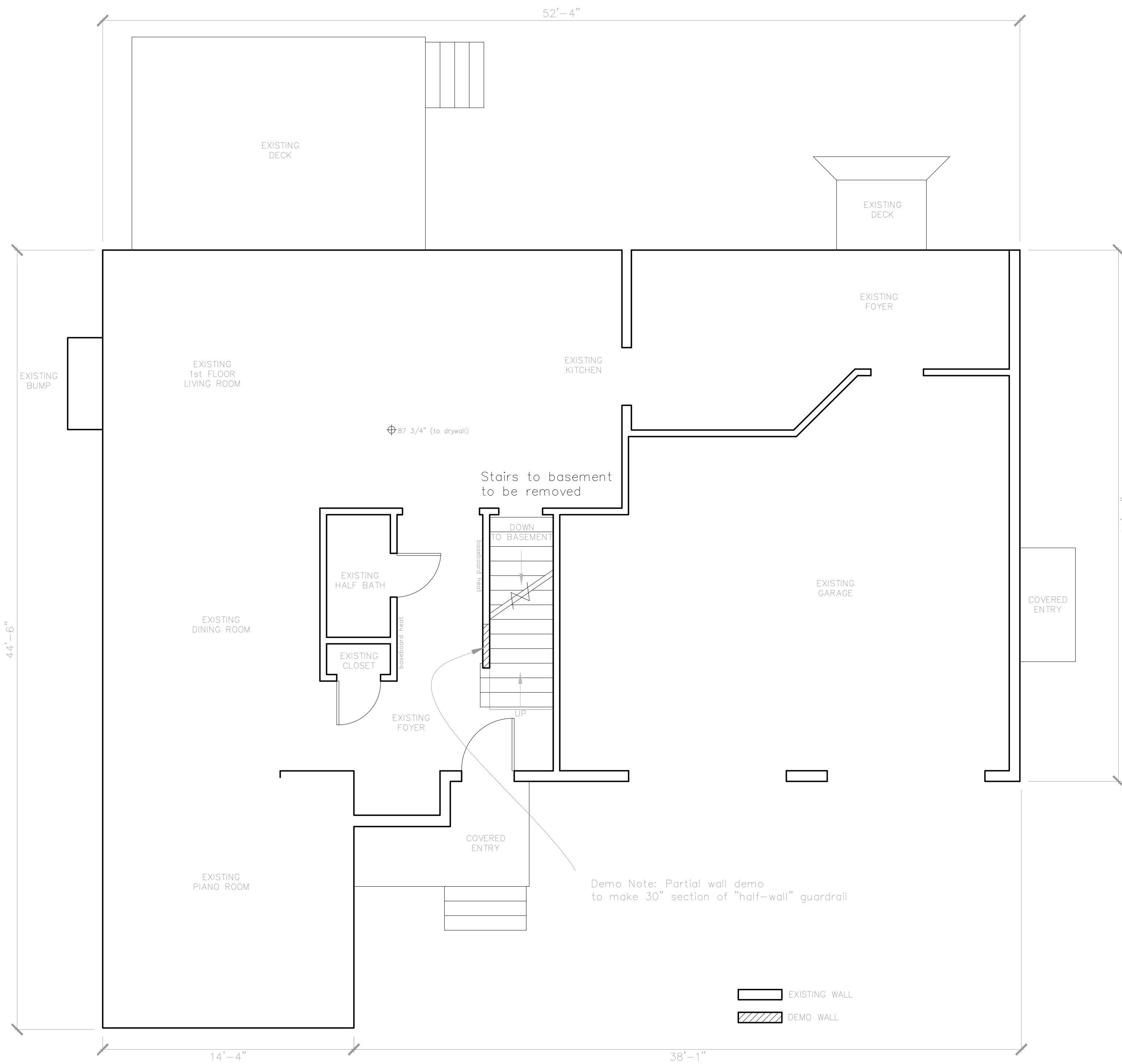
A Existing First Floor 1/4" = 1'-0"
