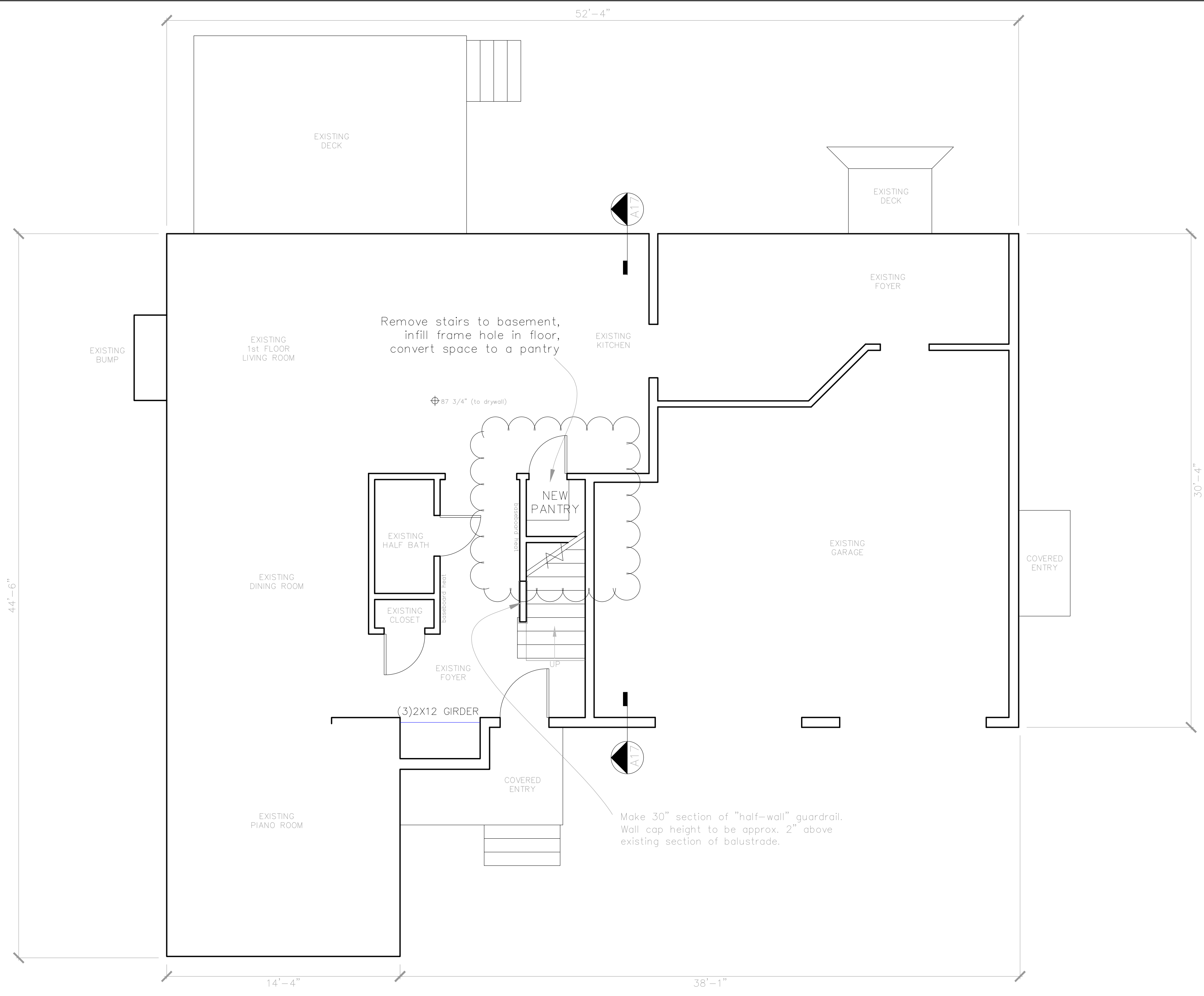
A Proposed First Floor 1/4" = 1'-0"
