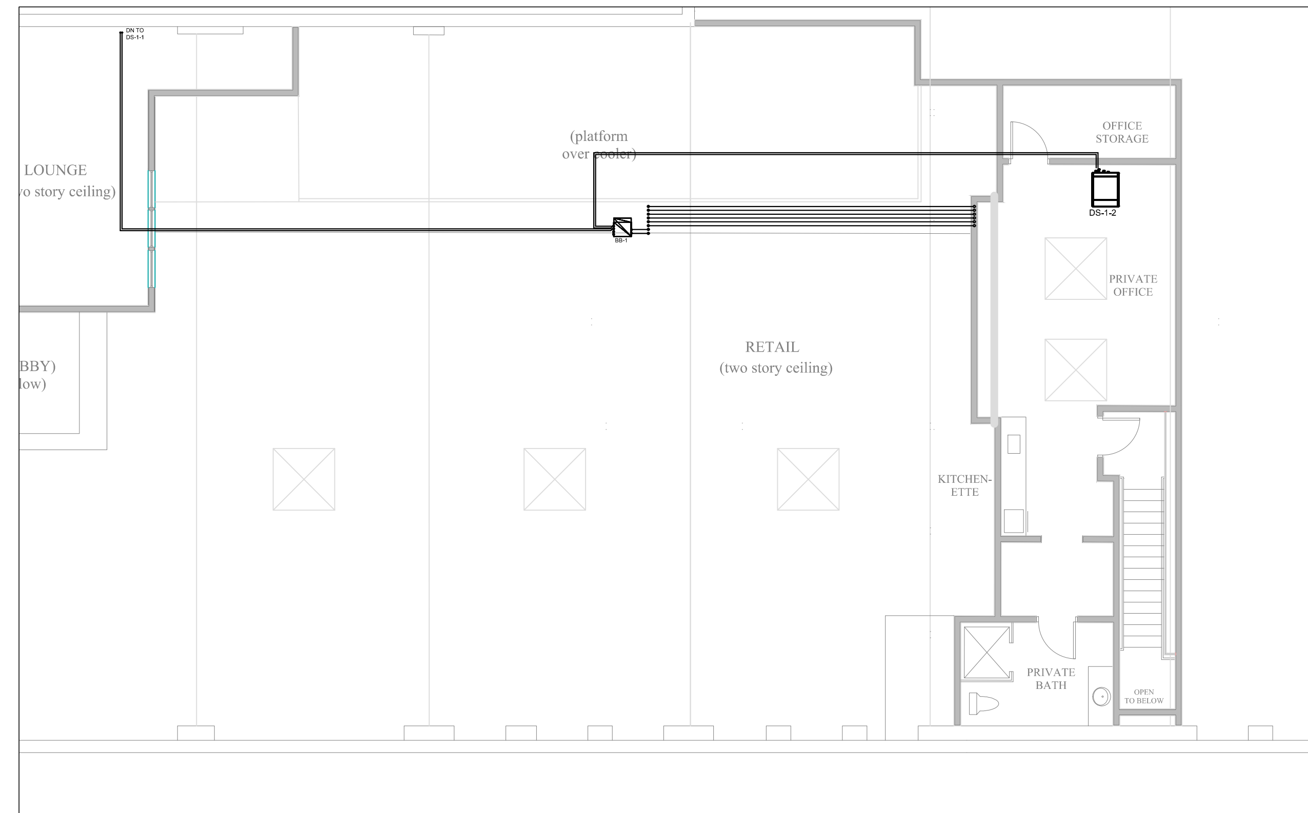
SECOND FLOOR PIPING PLAN SCALE: 1/8" = 1'-0"
