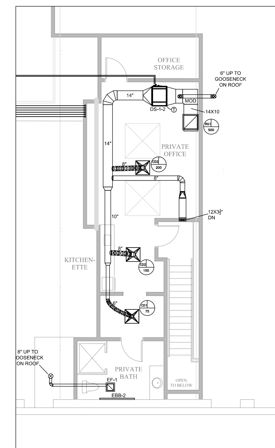
SECOND FLOOR HVAC PLAN SCALE: 1/8" = 1'-0"
