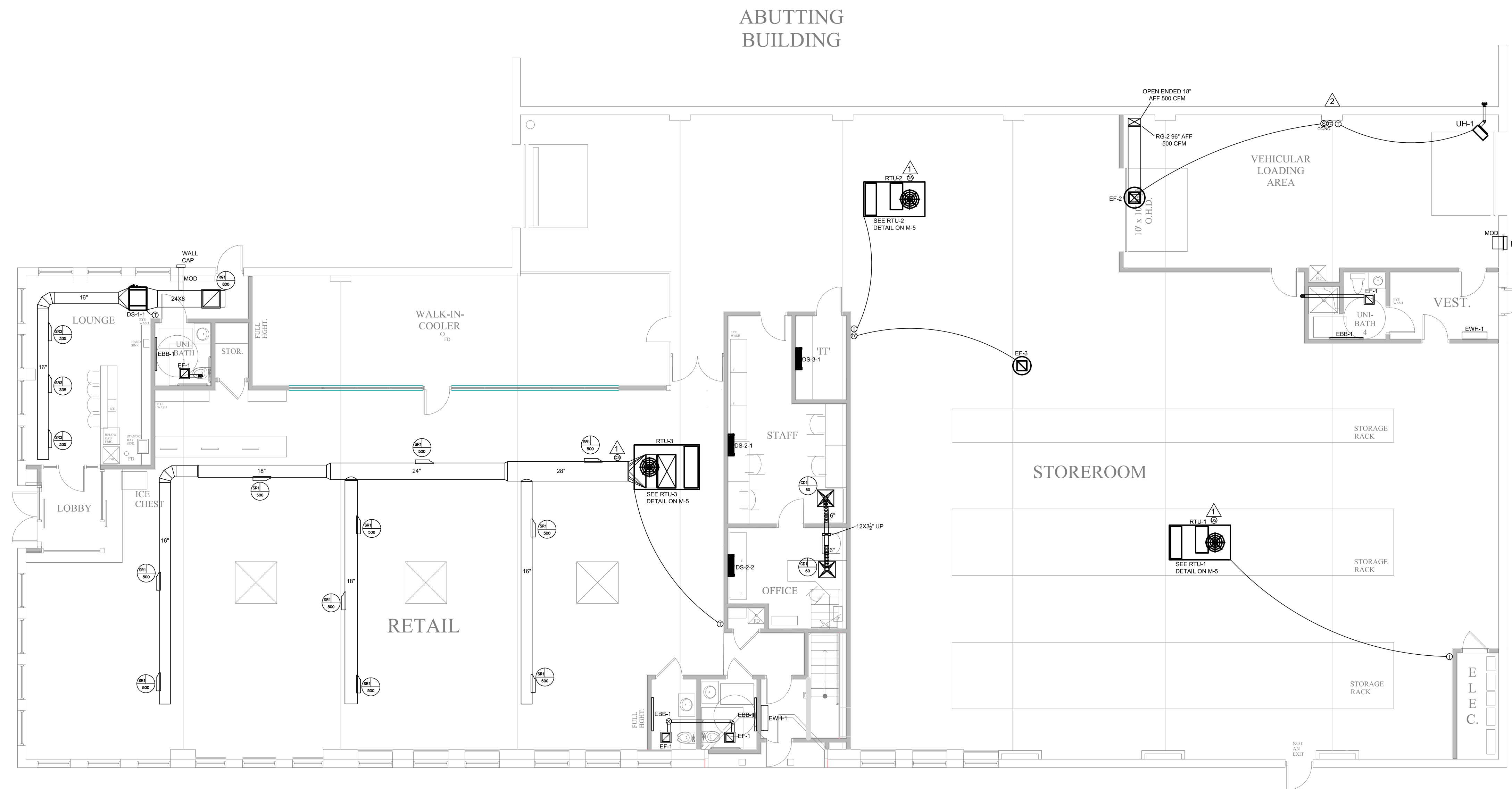
FIRST FLOOR HVAC PLAN SCALE: 1/8" = 1'-0"
