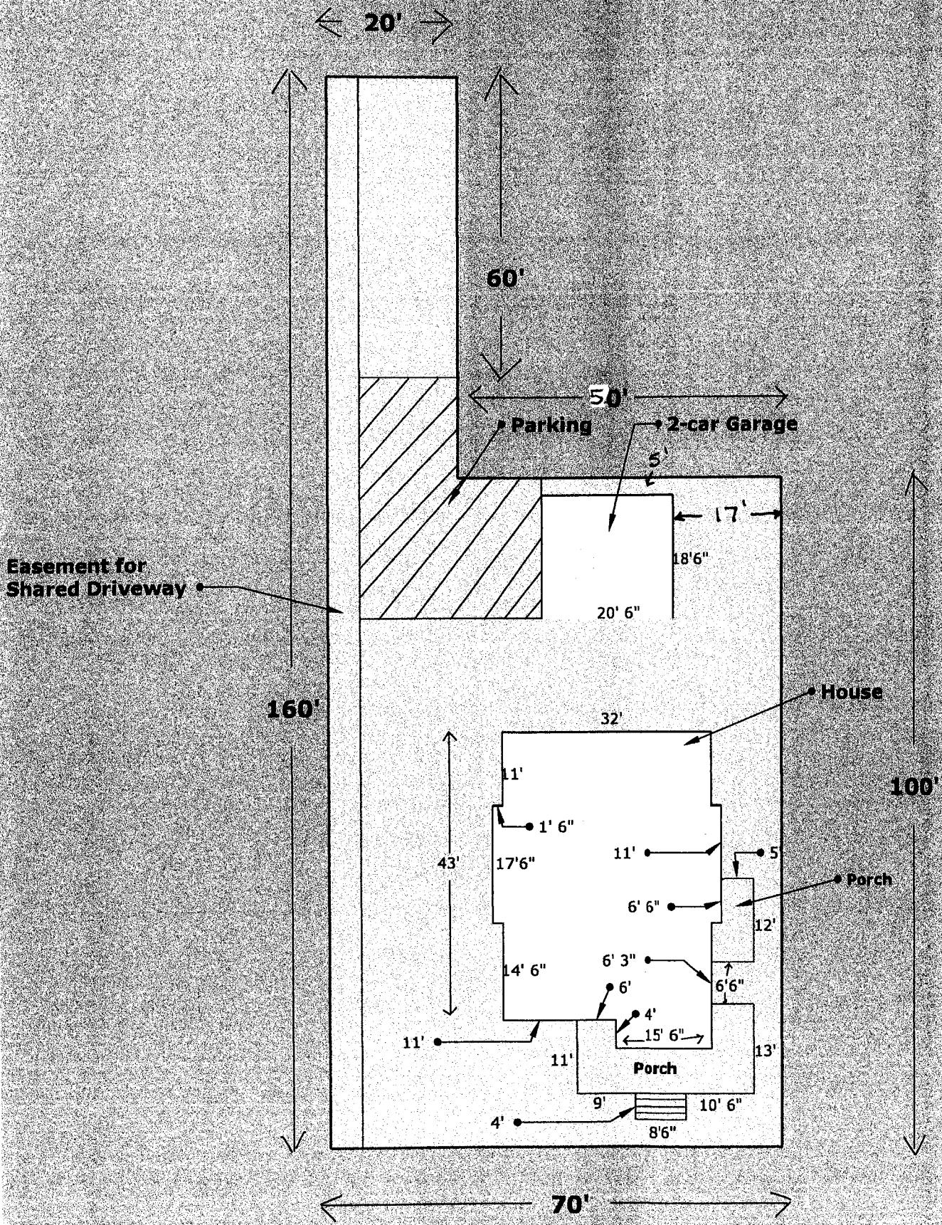
15 Longfellow Street Plot Plan
