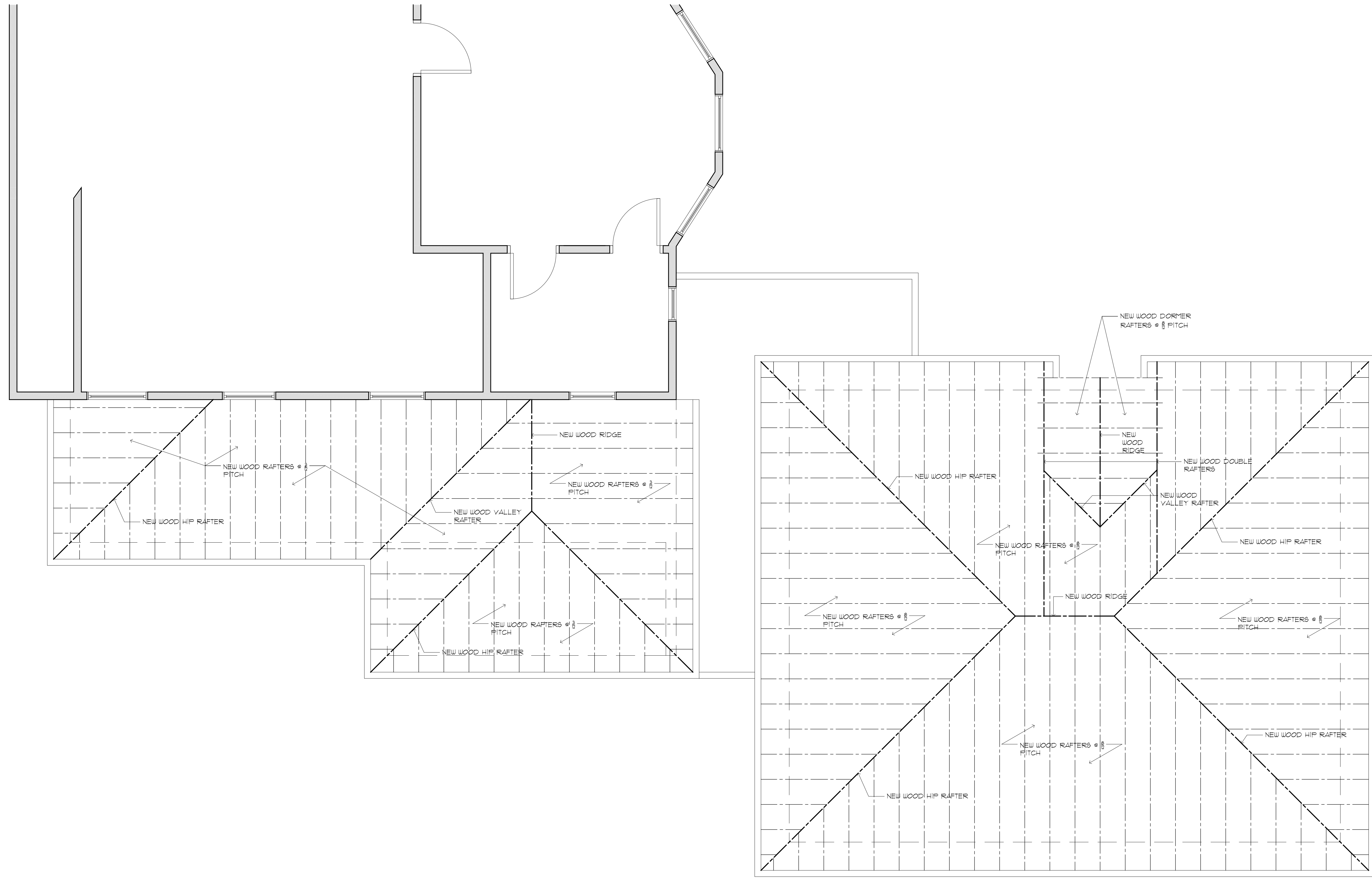
1 ROOF FRAMING PLAN S102 SCALE: 1/2"=1'-0"
