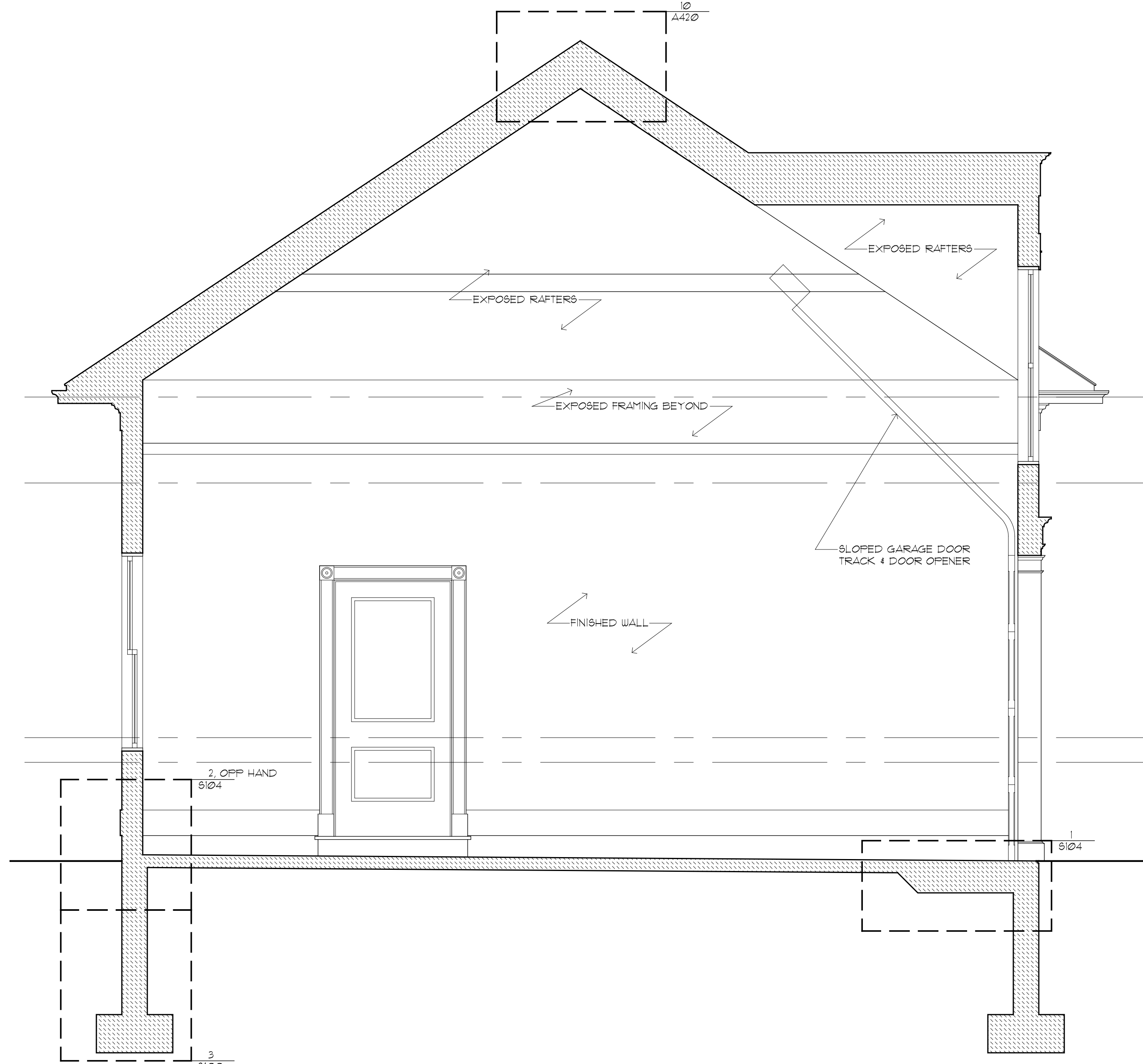
1 SECTION THROUGH GARAGE A301 SCALE: 1/2"=1'-0"
