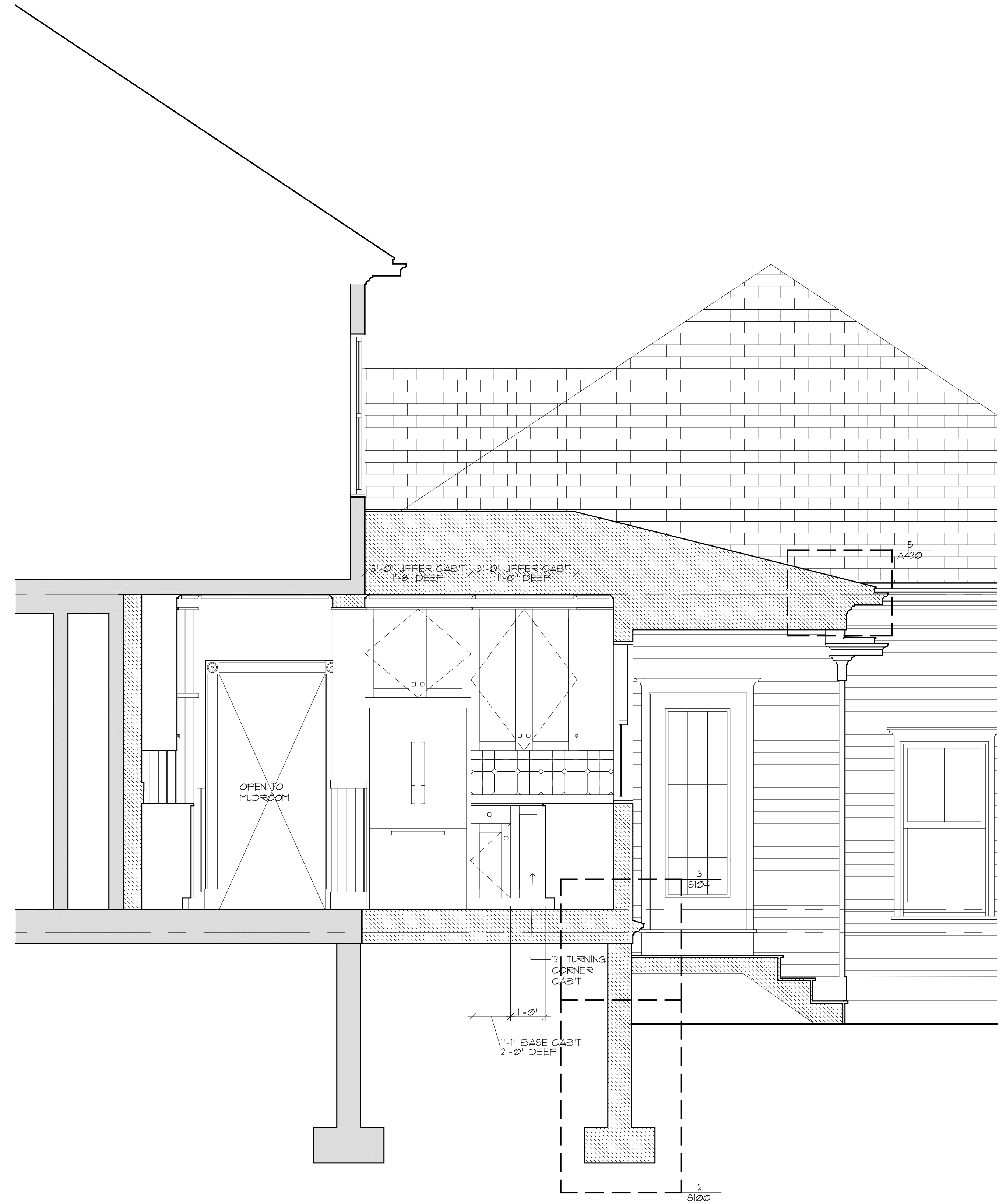
2 SECTION THROUGH KITCHEN / PORCH A300 SCALE: 1/2"=1'-0"
