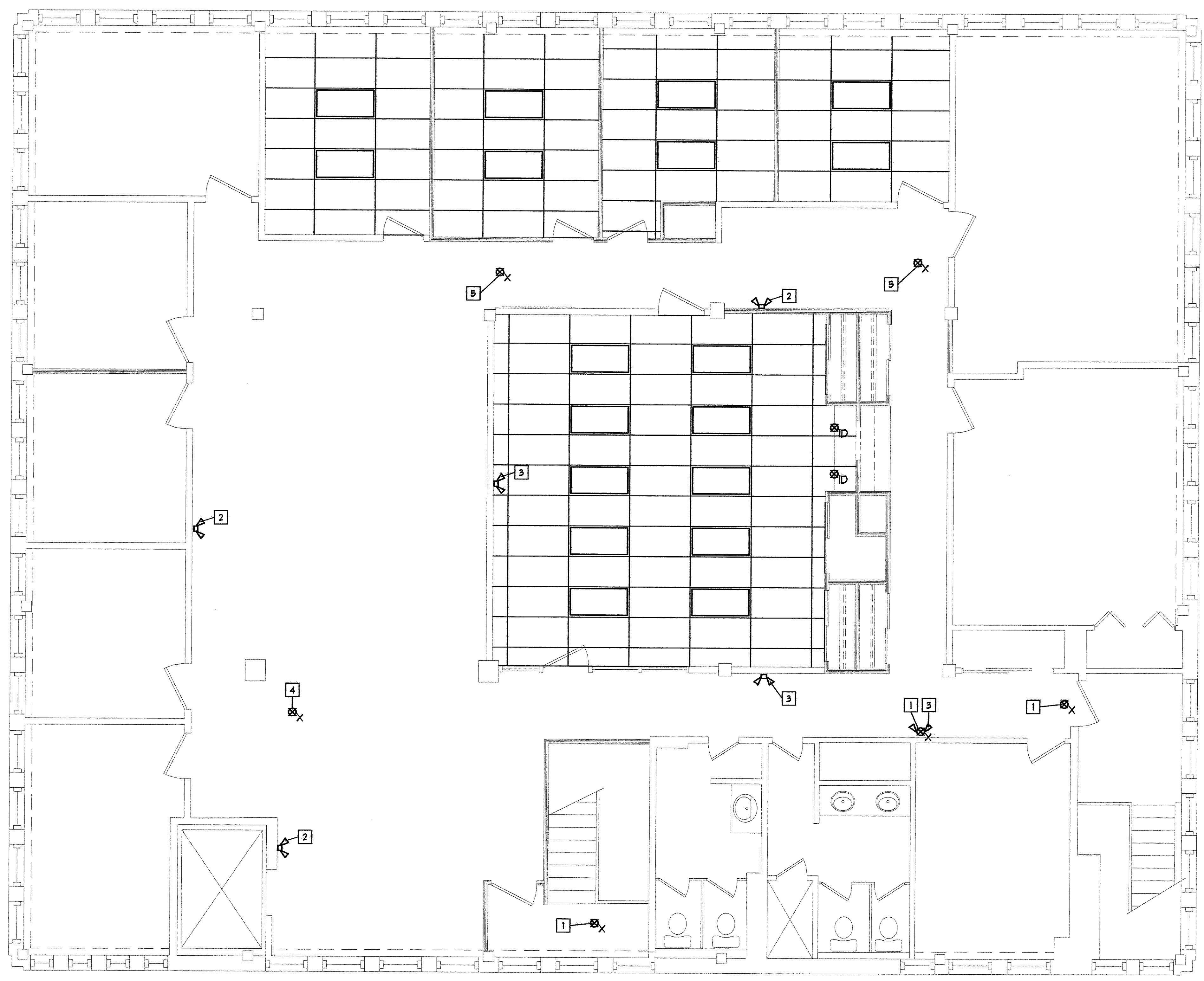
REFLECTED CEILING PLAN - 2nd FLOOR SCALE: 1/4" = 1'-0"
