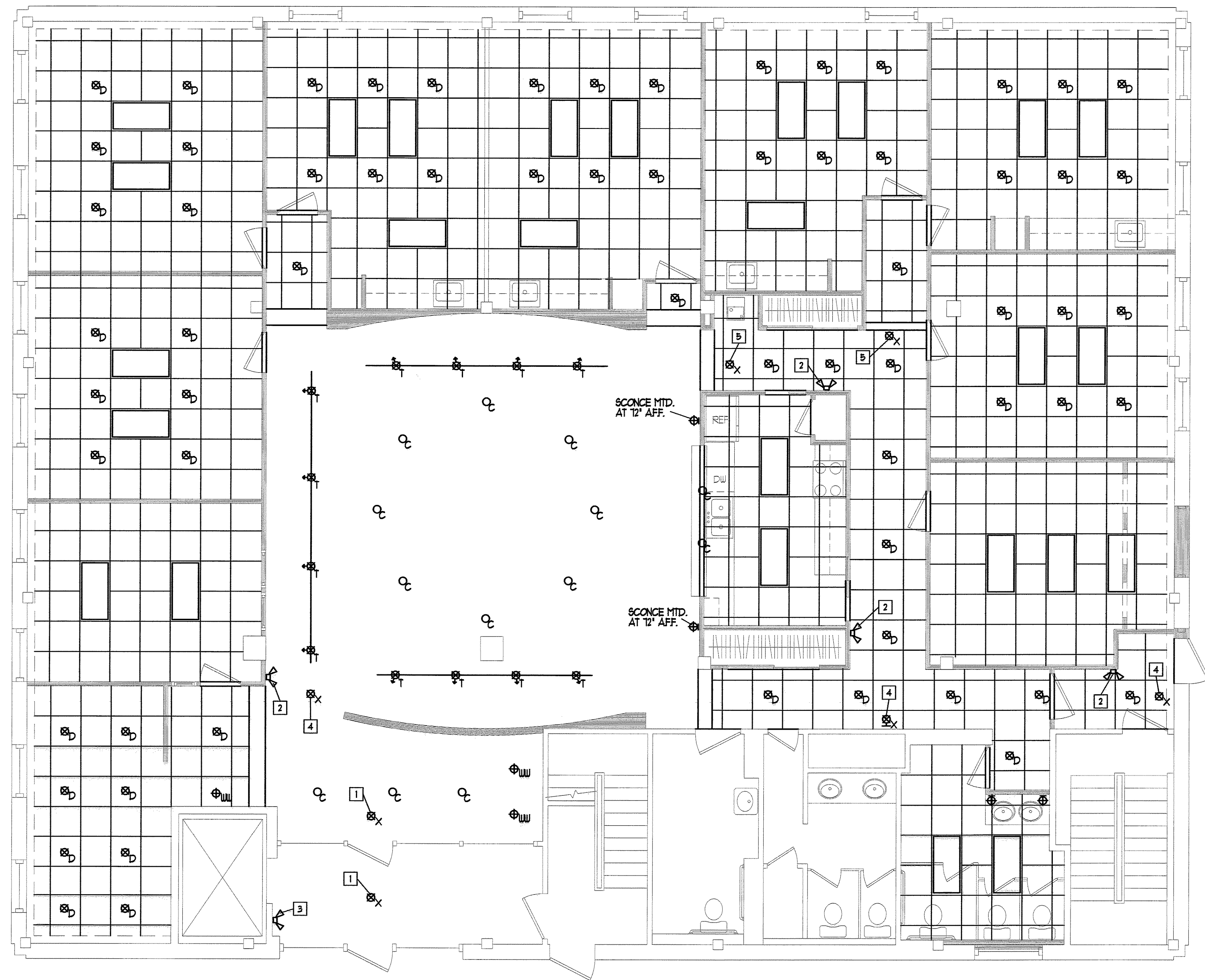
REFLECTED CEILING PLAN - 1st FLOOR SCALE: 1/4" = 1'-0"
