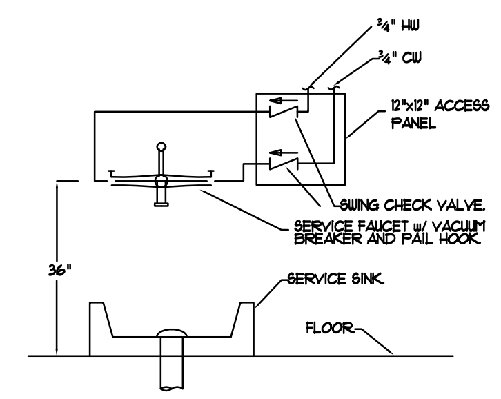
MOP BASIN INSTALLATION DETAIL NT6
