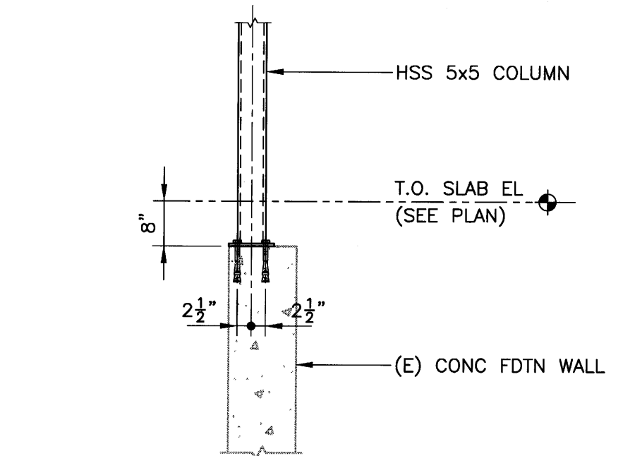
10 SECTION S1 SCALE: 1/2"=1'-0"
