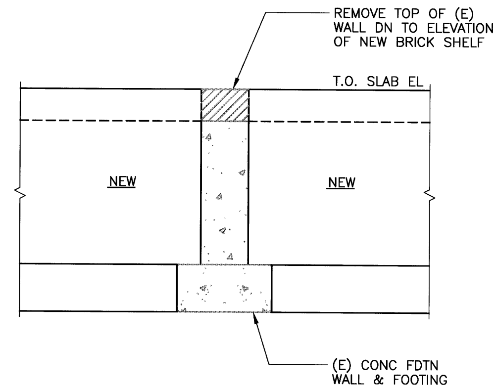
12 SECTION S1 SCALE: 1/2"=1'-0"
