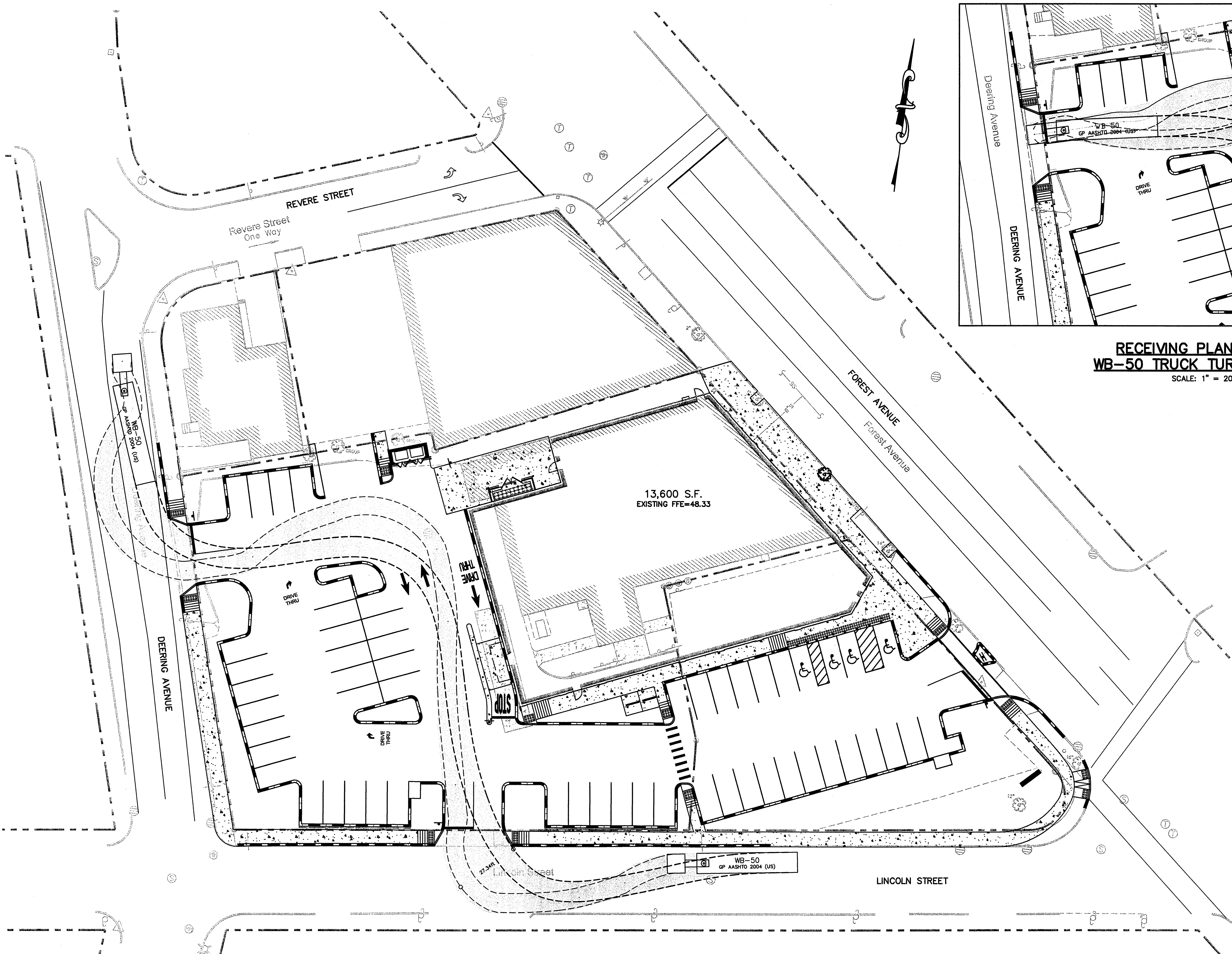
ACCESS EGRESS PLAN DETAIL WB-50 TRUCK TURNING PATH SCALE: 1" = 20'
