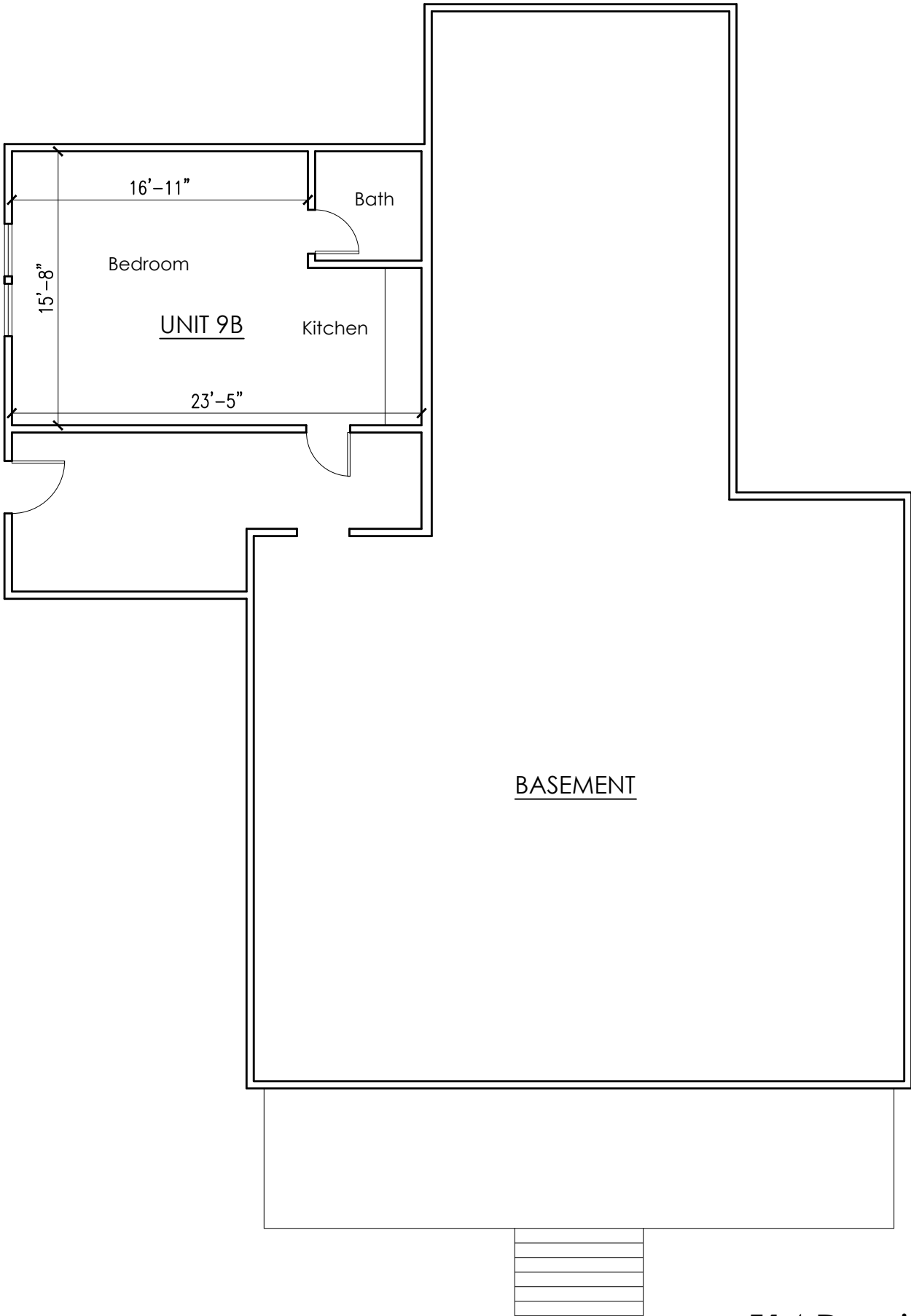
BASEMENT LEVEL PLAN scale: 1/8" = 1'-0"
