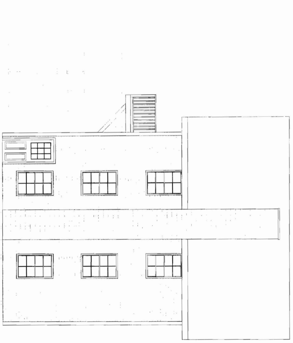
RIGHT 1/4" SCALE
