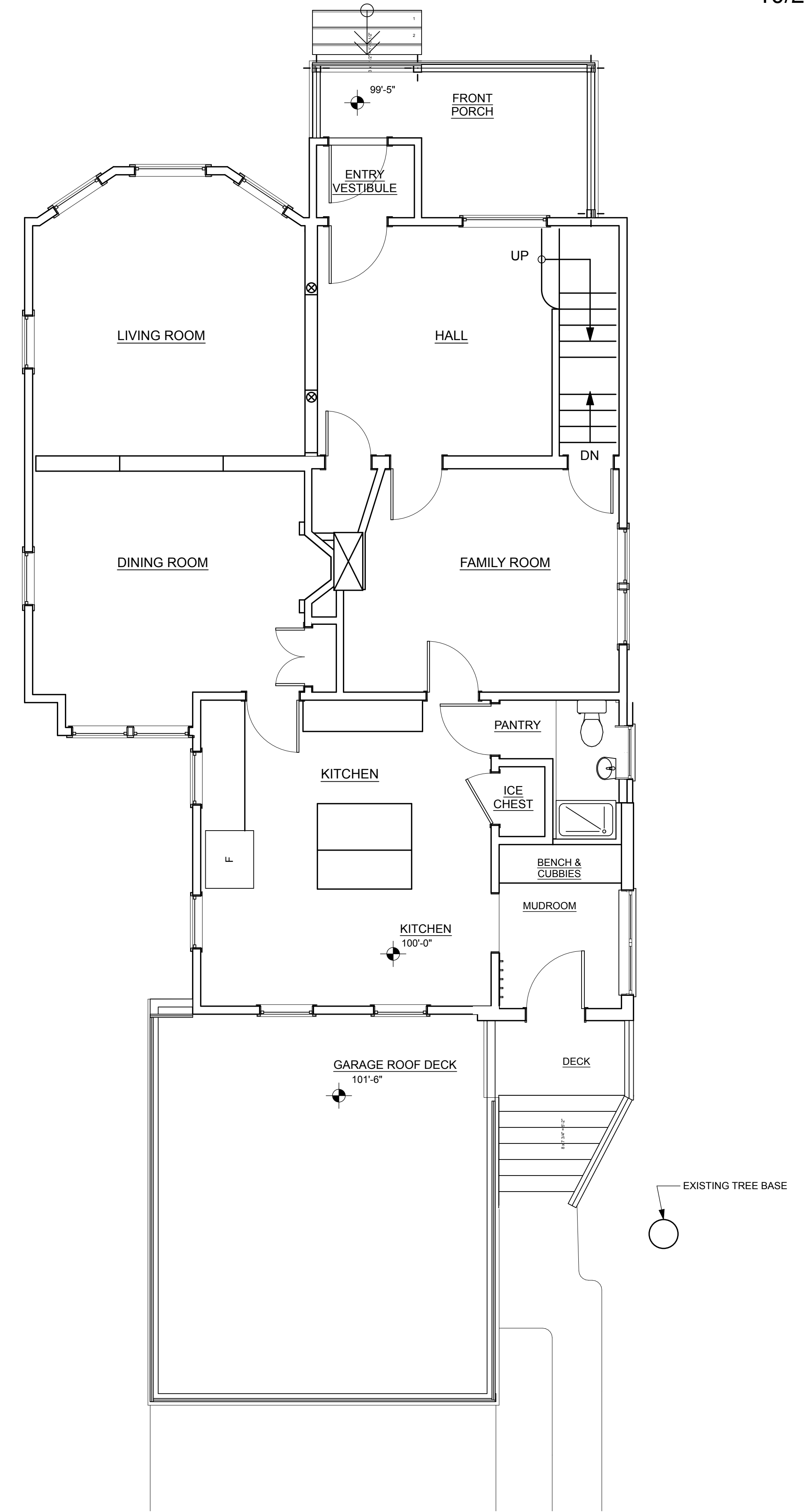
1 1st FLOOR SCALE: 1/4" = 1'-0"
