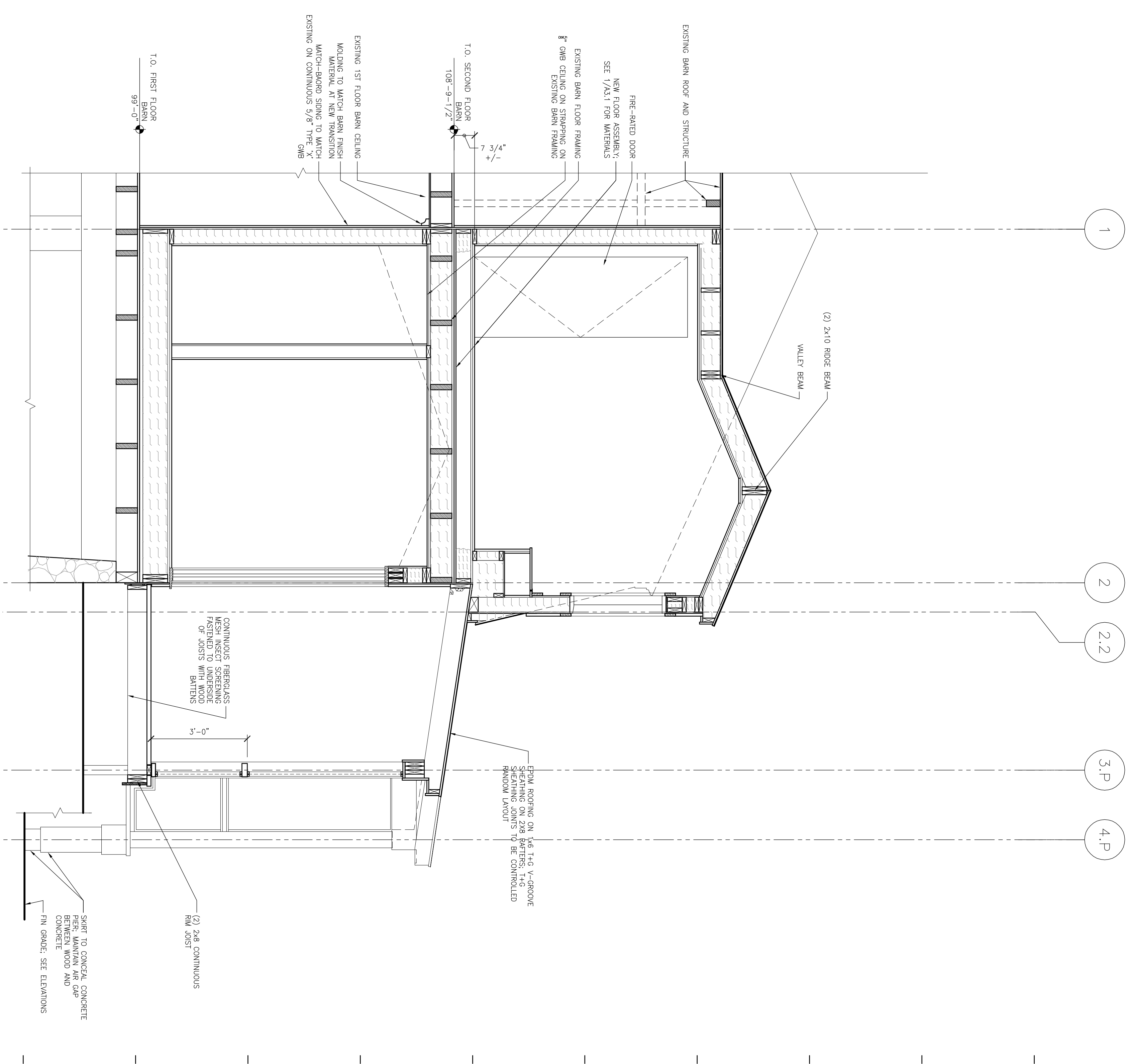
1 SECTION THROUGH NEW WORK 1/2" = 1'-0"
