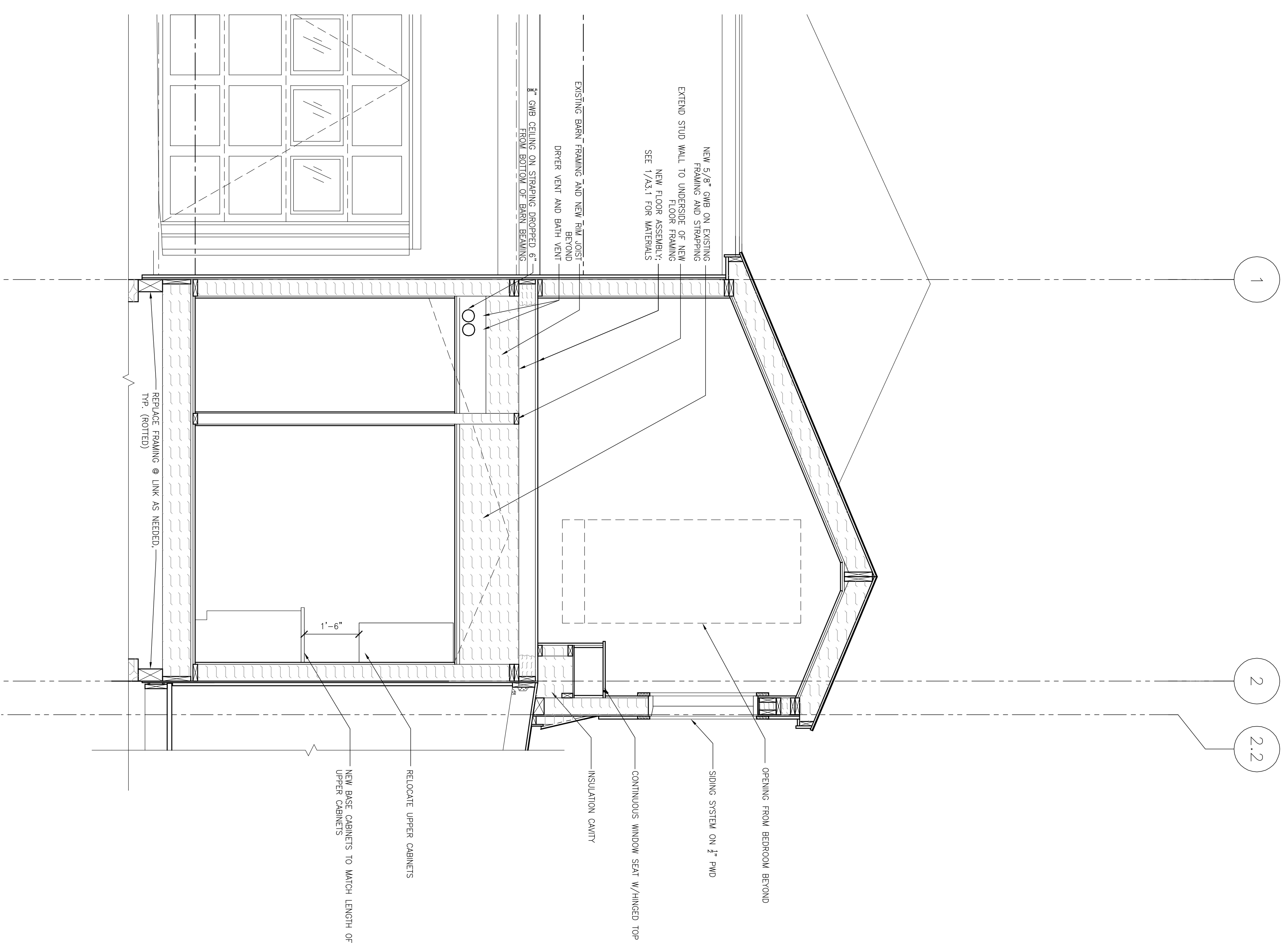
1 SECTION THROUGH LINK BETWEEN BARN AND HOUSE 1/2" = 1'-0"
