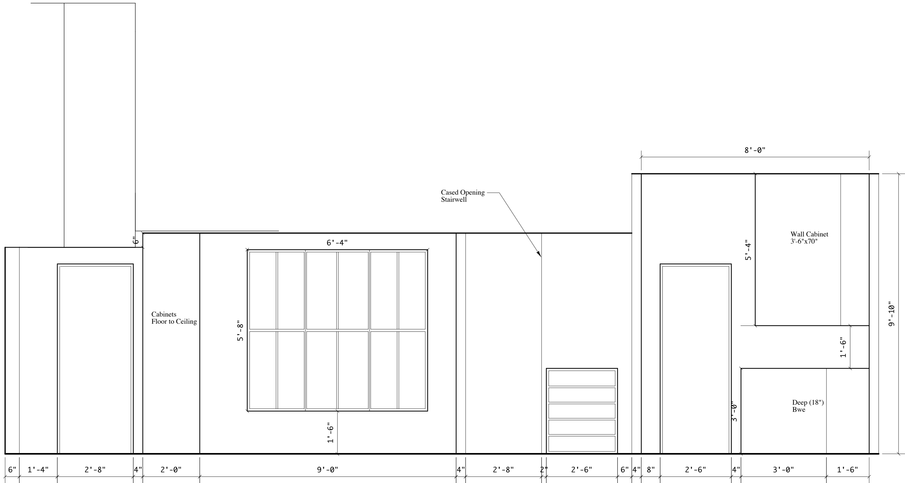
Elevation: C Rob & Beth Revenelle 2012 Scale: 1/2"=1'-0"
