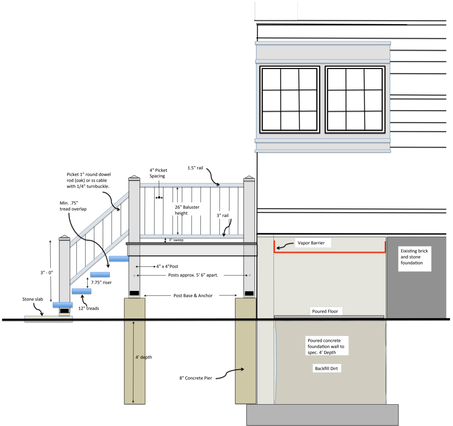
PROPOSED FOUNDATION PORCH PLAN WITH STAIR DETAIL VIEW FACING SIDE OF HOUSE
