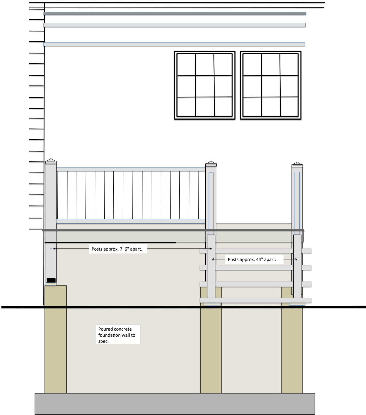
PROPOSED FOUNDATION PORCH PLAN VIEW FACING BACK OF HOUSE
