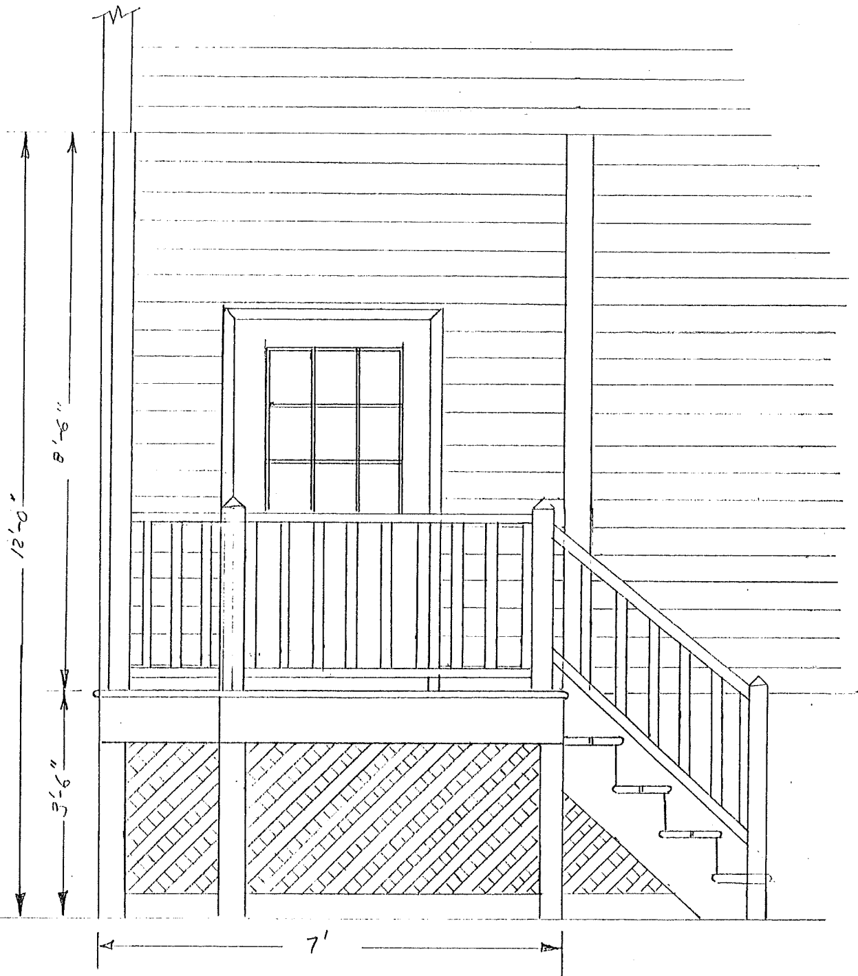
SIDE ELEVATION
