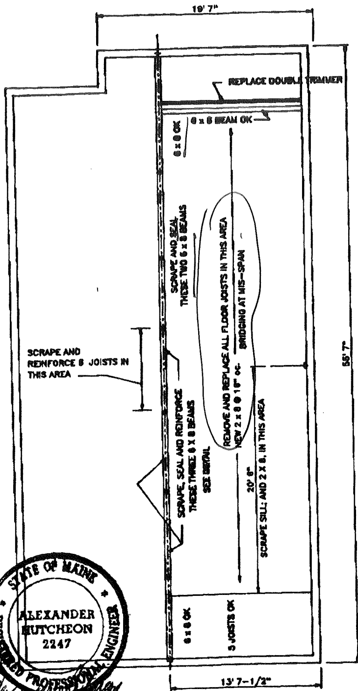
FIRST FLOOR FRAMING PLAN
