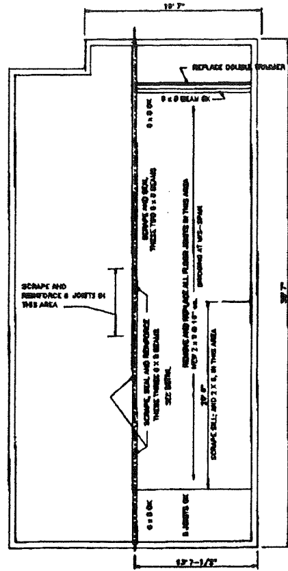
FIRST FLOOR FRAMING PLAN
