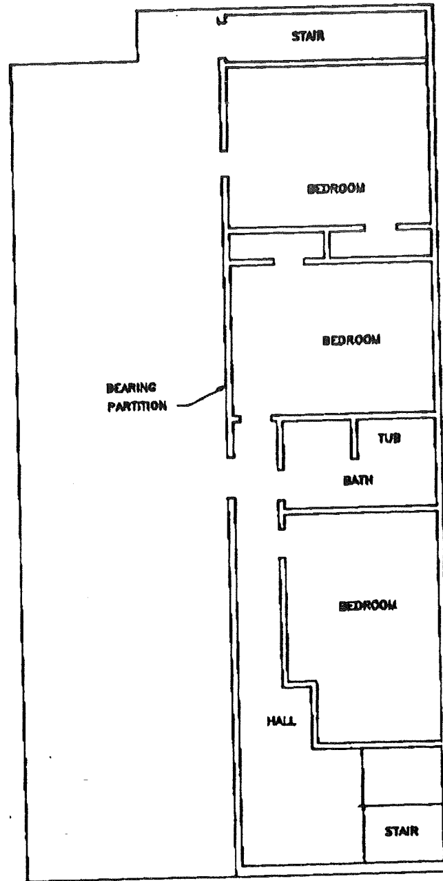
FIRST FLOOR PARTITION PLAN
