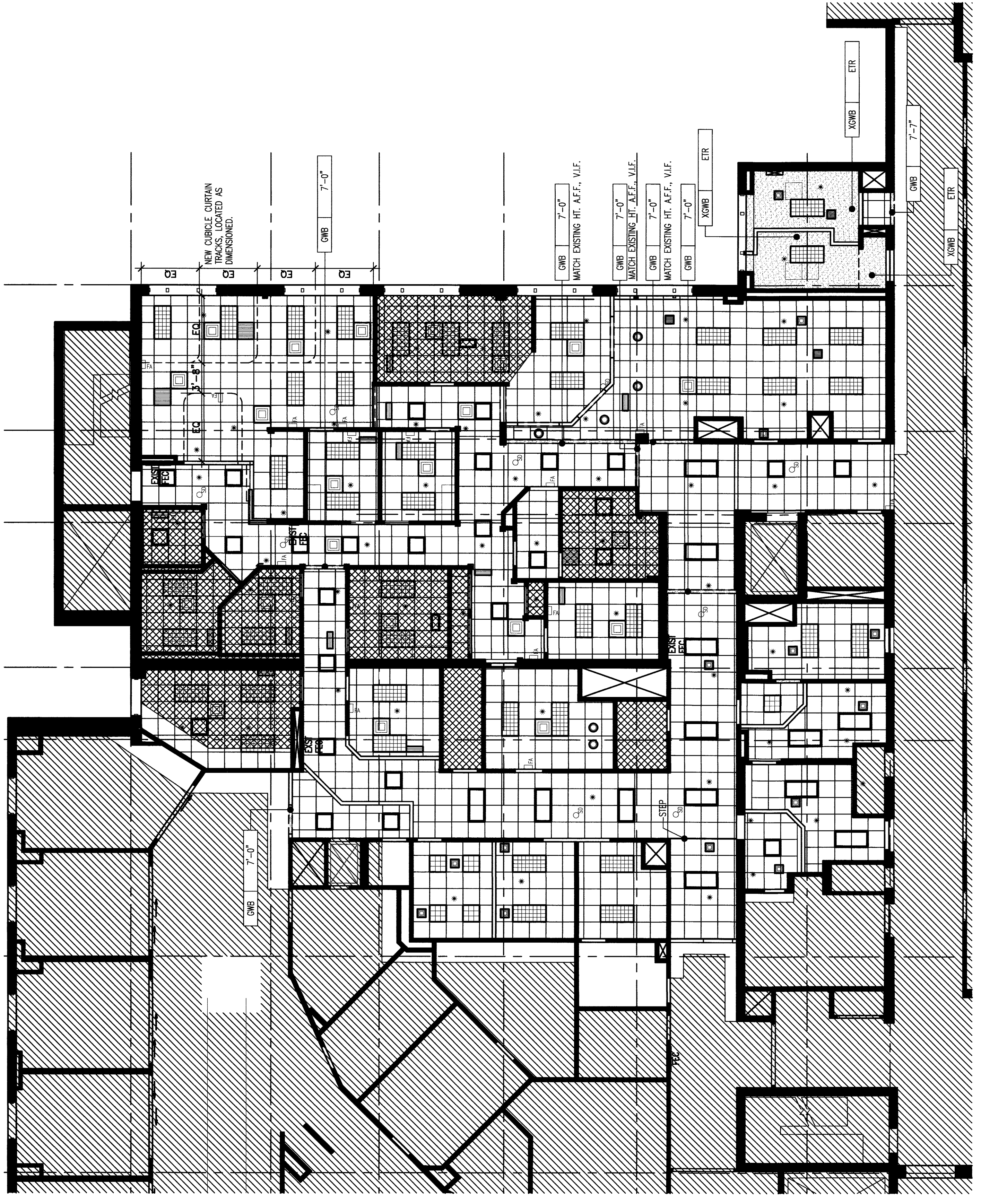
1 SECOND FLOOR REFLECTED CEILING PLAN 1/8" = 1'-0"
