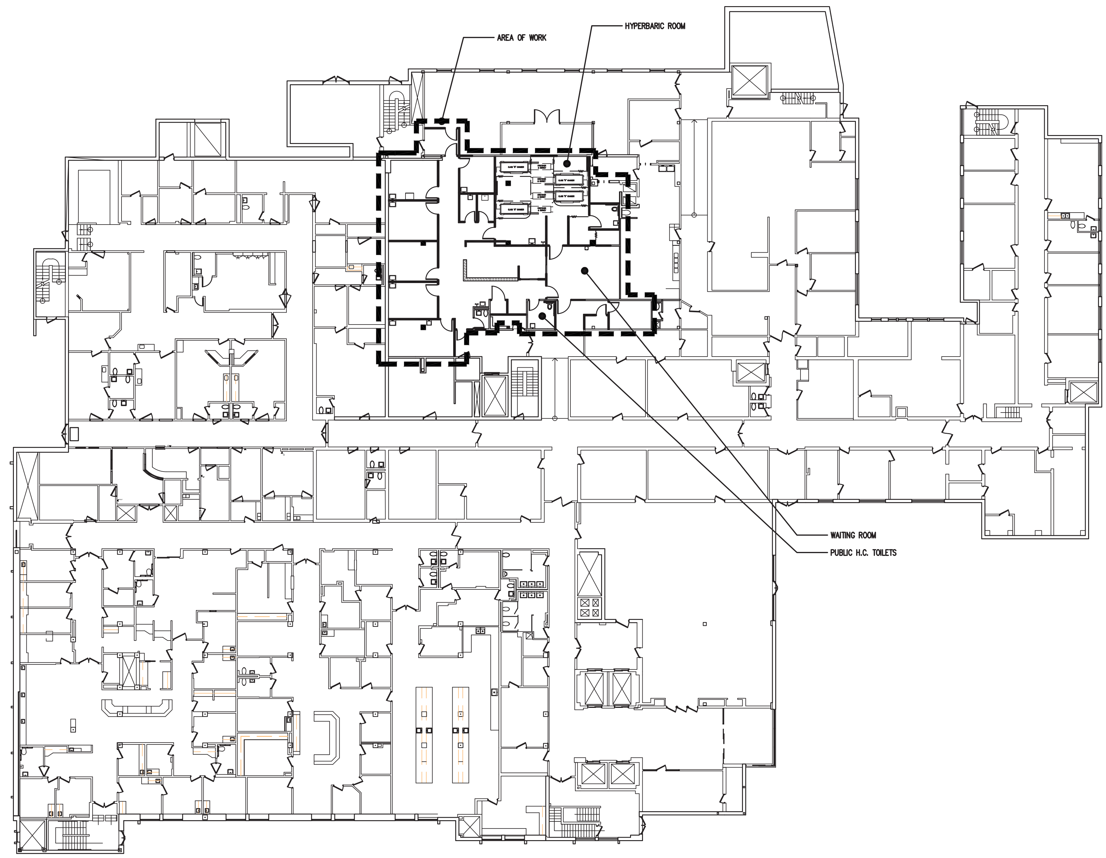
1 Full Floor Plan
