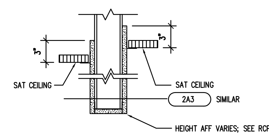
3 TYP. GWB SOFFIT DETAIL 1 1/2" = 1'-0"
